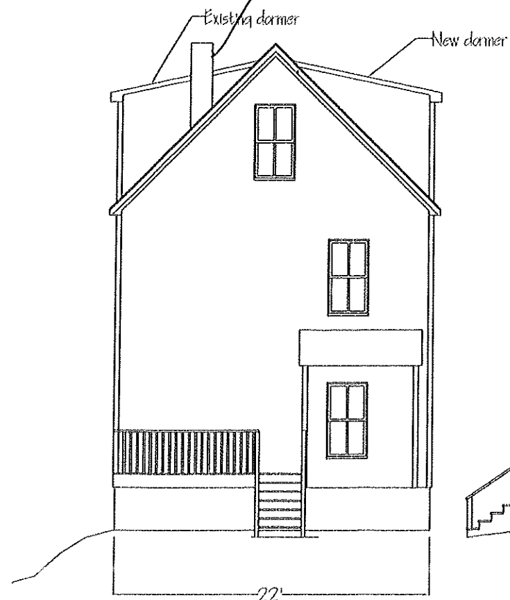
West Elevation (Rear)
