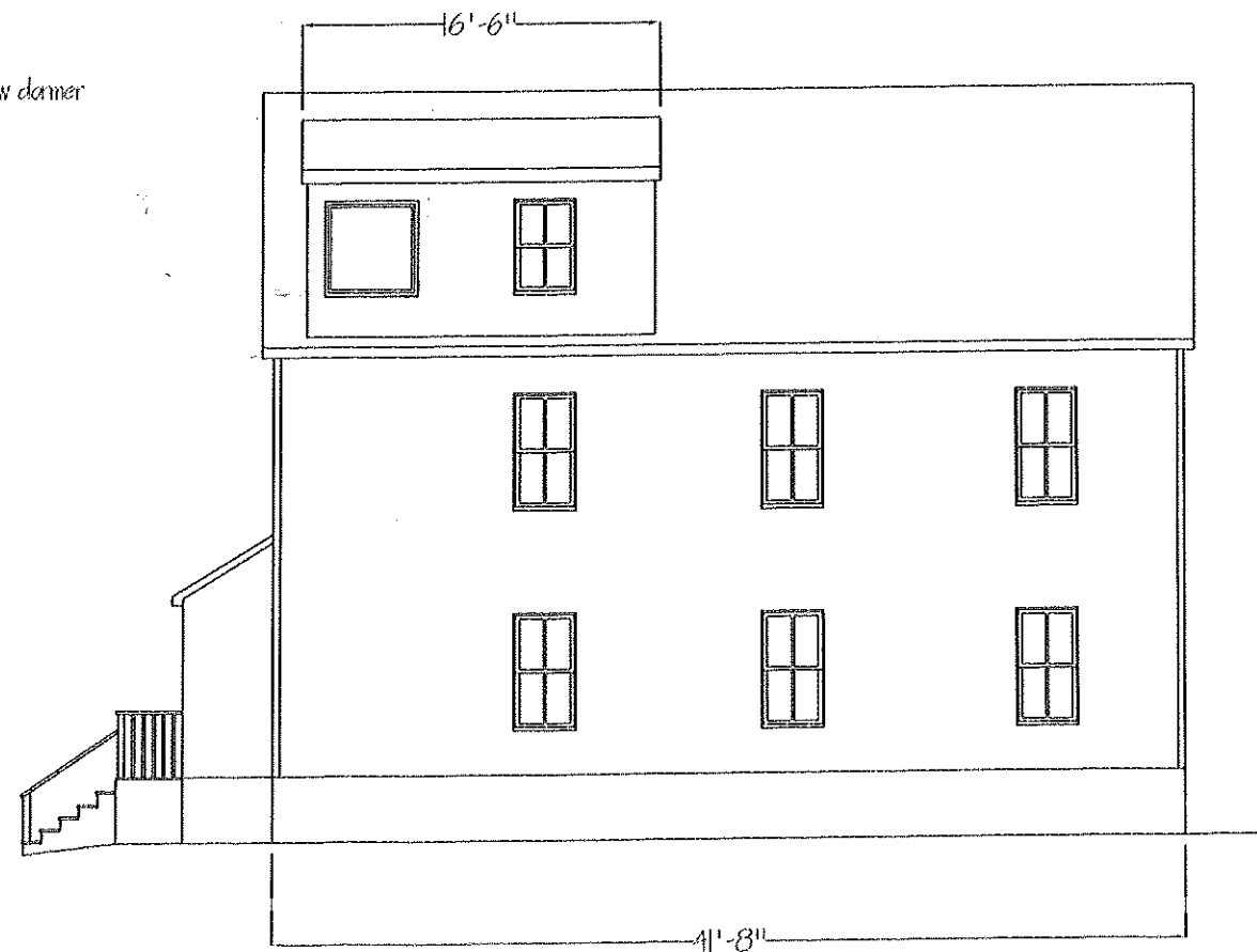
South Elevation
