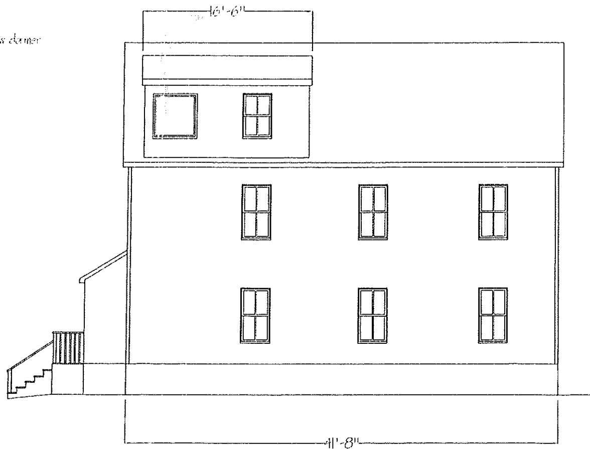
South Elevation
