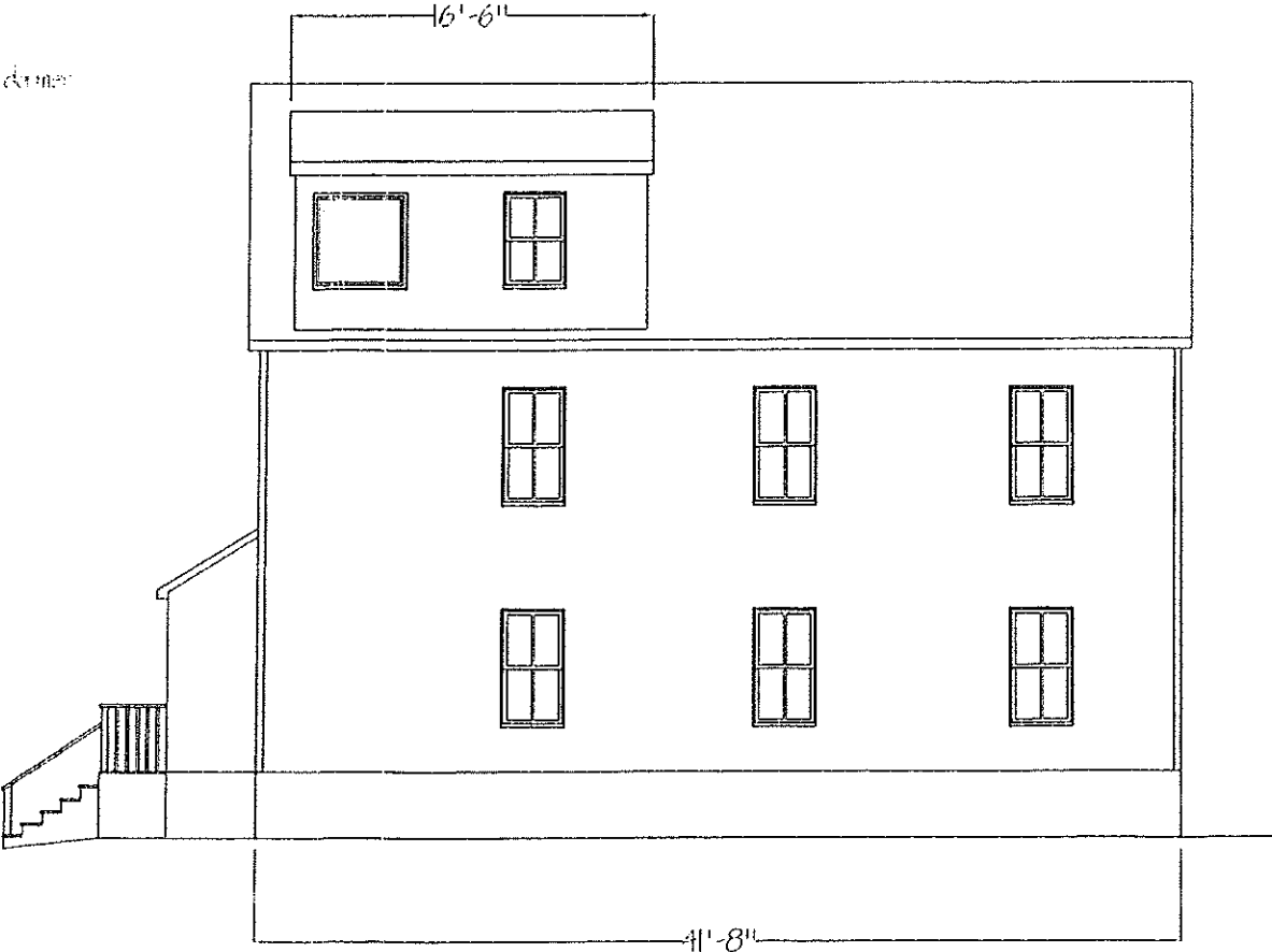
South Elevation
