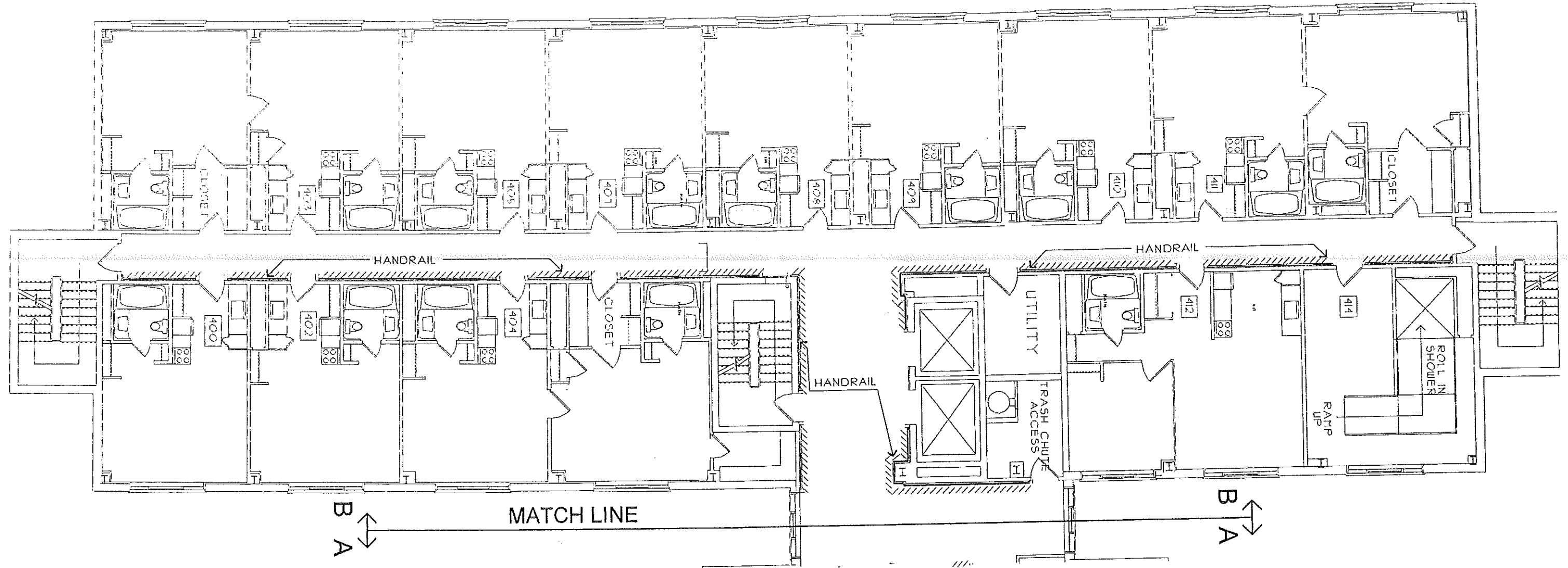
FLOOR 4/5/6 HARBOR TERRACE PORTLAND HOUSING AUTHORITY HANDRAIL LAYOUT
