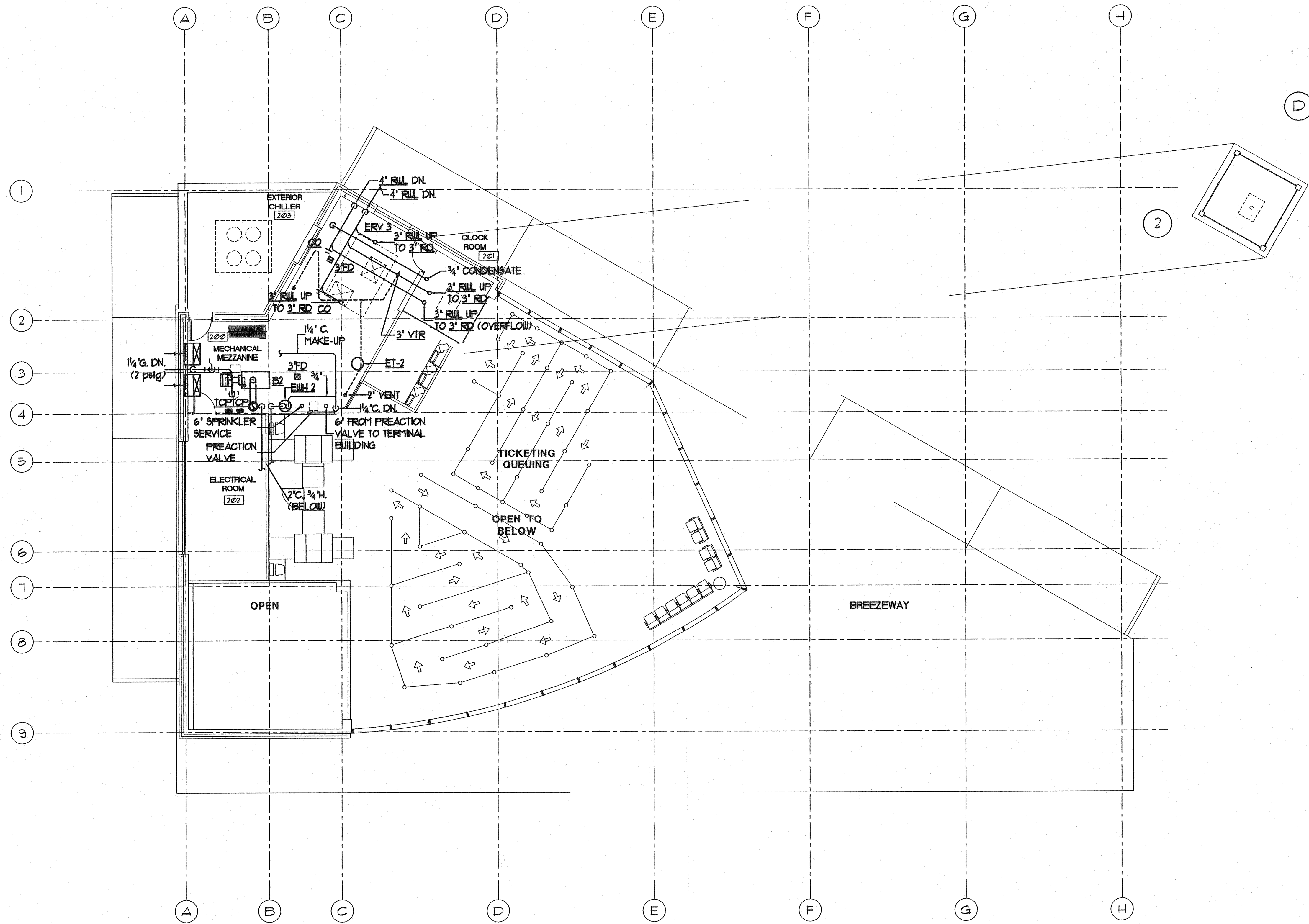
RECEIVING STATION GROUND FLOOR PLAN SCALE: 1/8"=1'-0"
