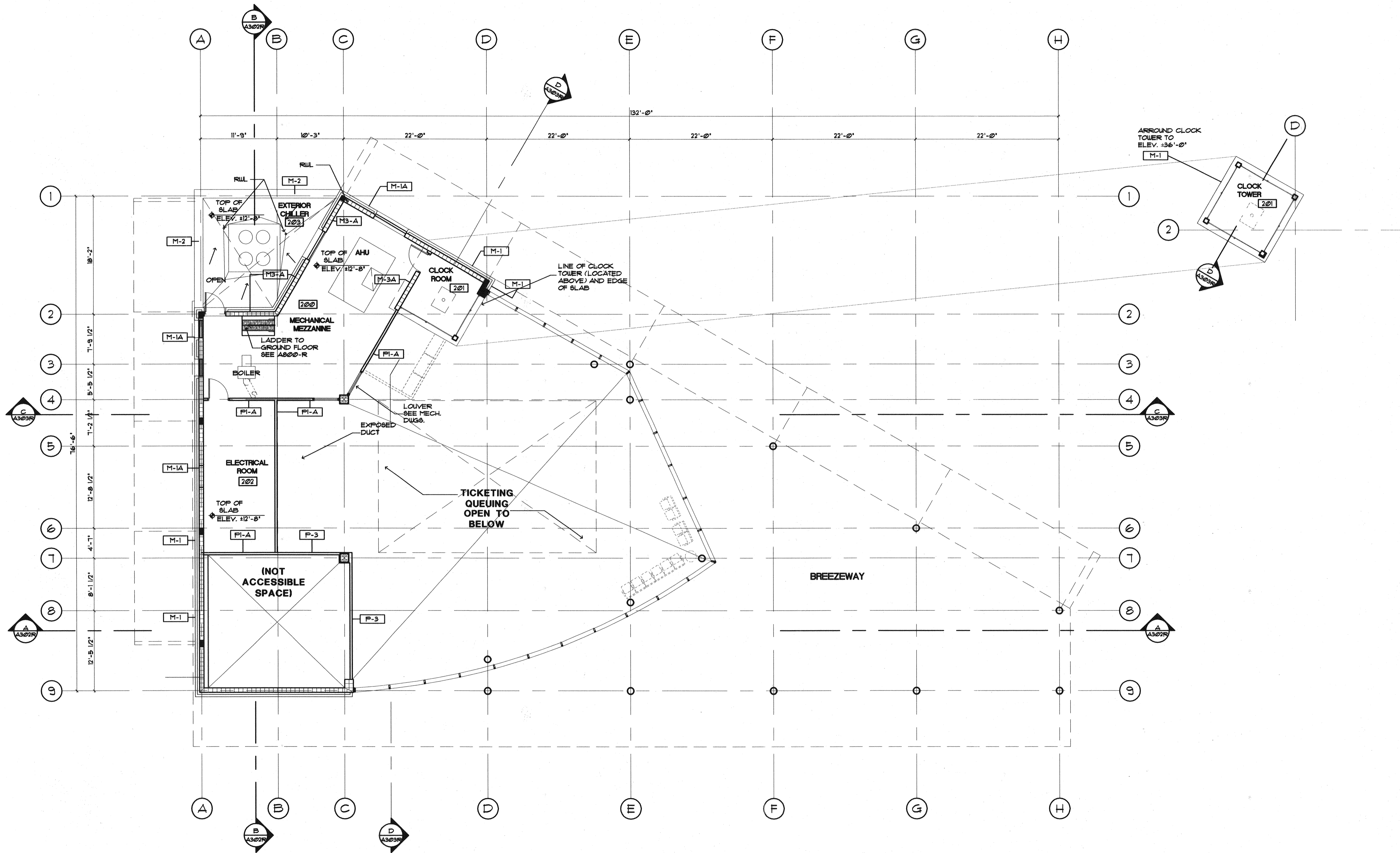
MEZZANINE PLAN PARTITION TYPE PLAN SCALE: 1/8"=1'-0"
