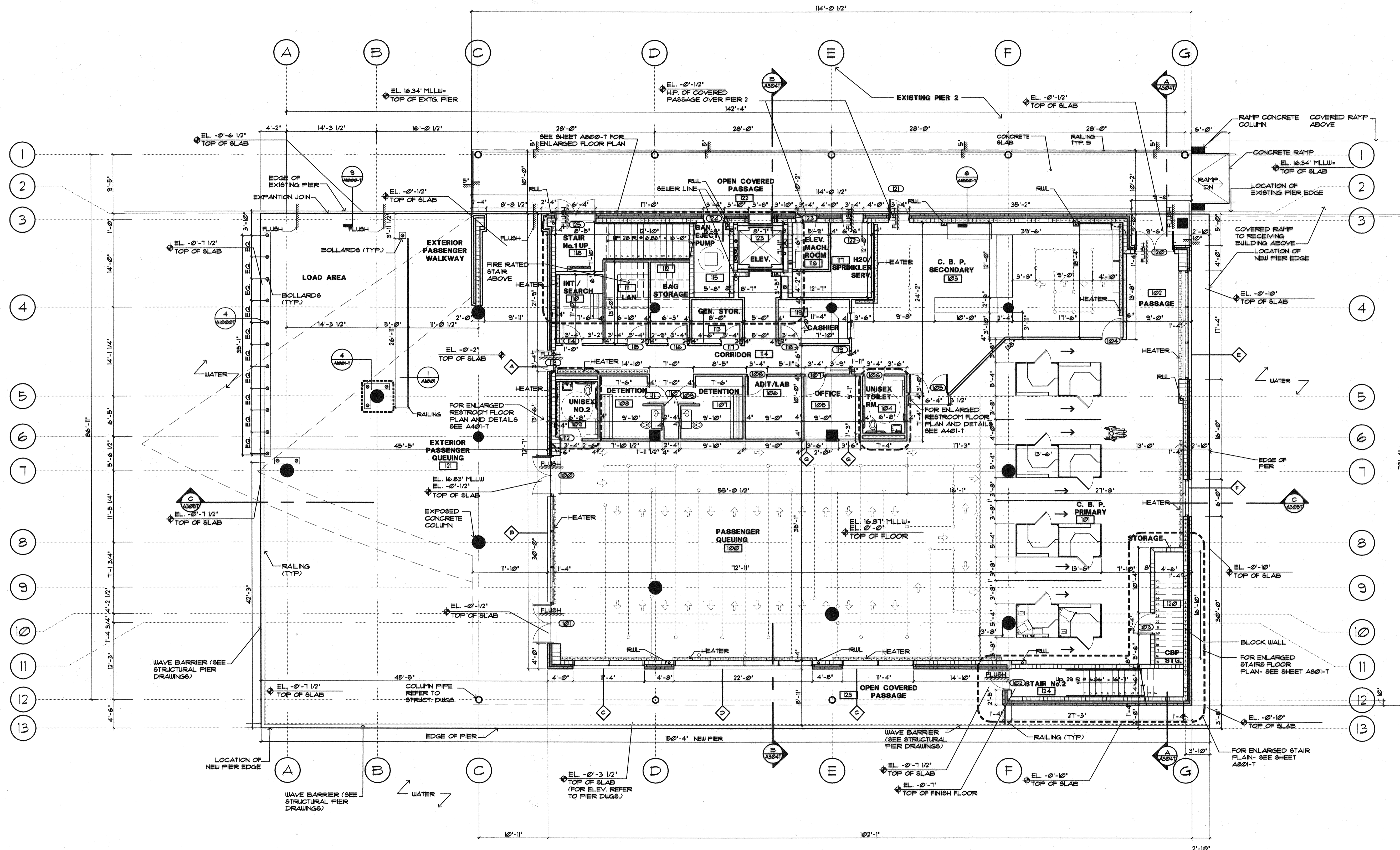
FIRST LEVEL PLAN SCALE: 1/8" = 1'-0"
