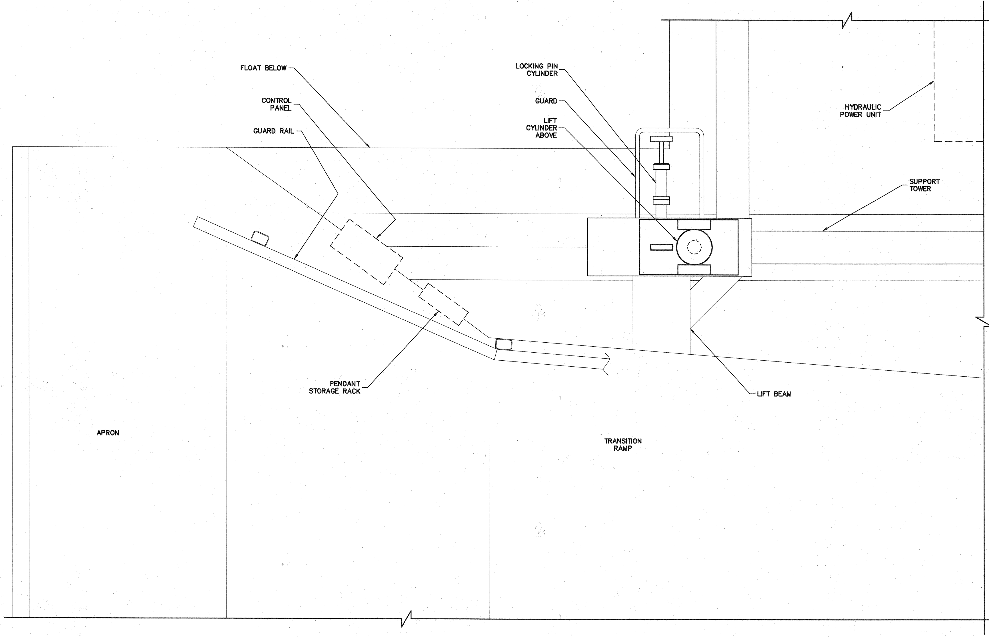
GENERAL ARRANGEMENT PLAN MECHANICAL SYSTEM
