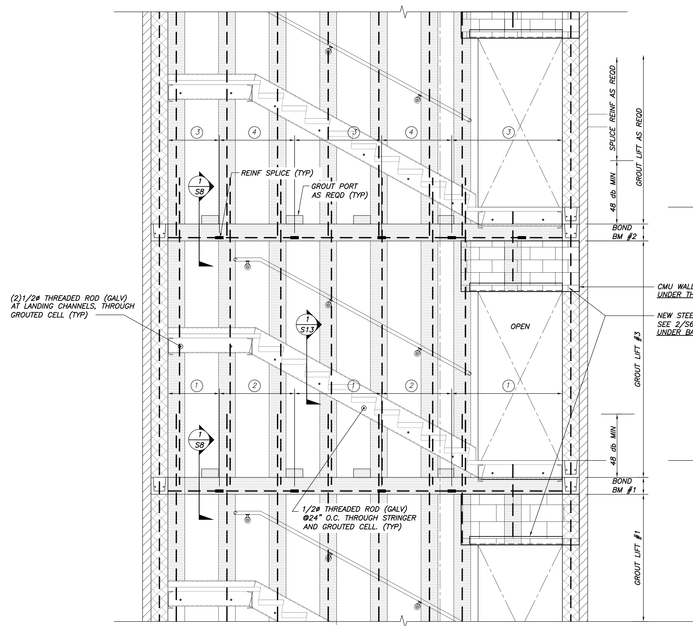
DETAIL B 1/2"=1'-0" S10
