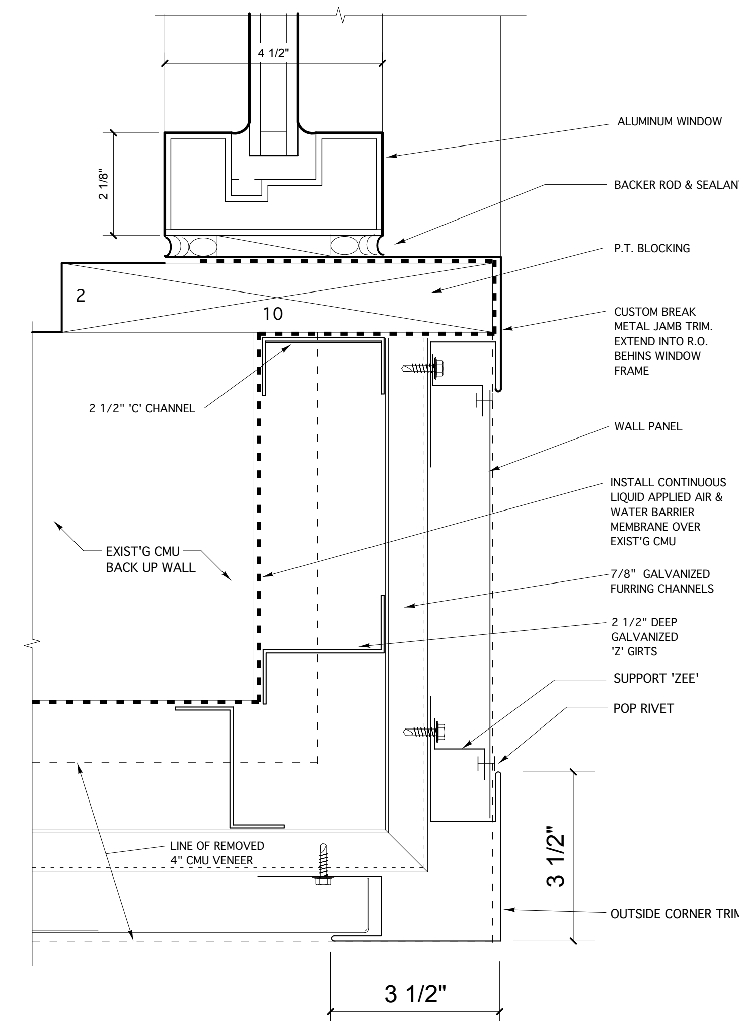
16 WINDOW JAMB DETAIL 6"=1'-0"
