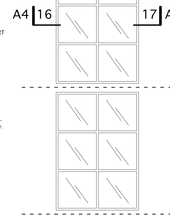
17 FIXED FRAME UNIT 17 Units Req'd
