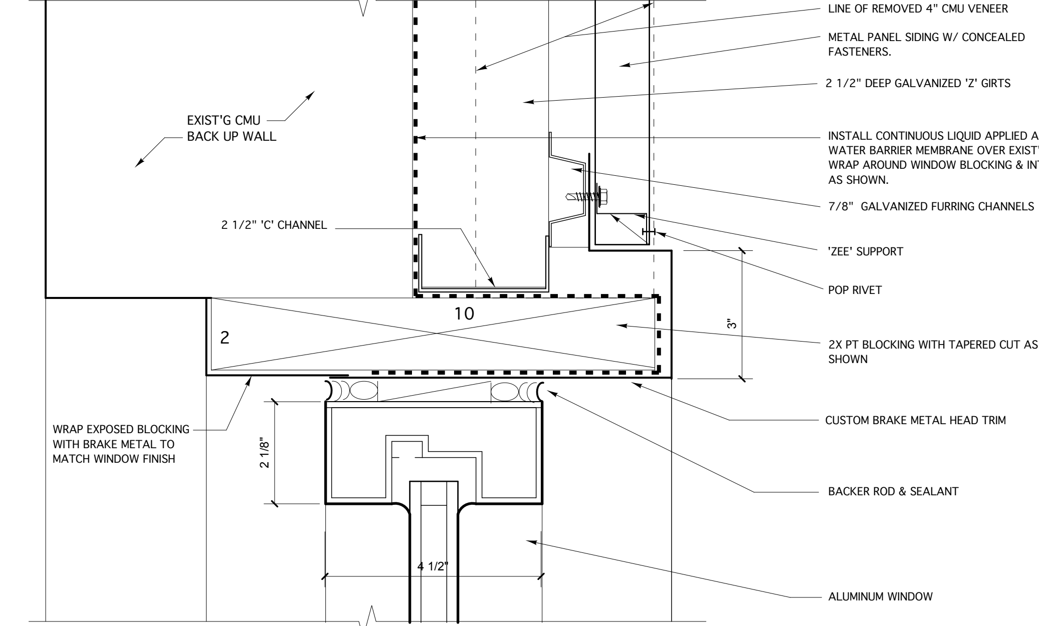
15 WINDOW HEAD DETAIL 6"=1'-0"
