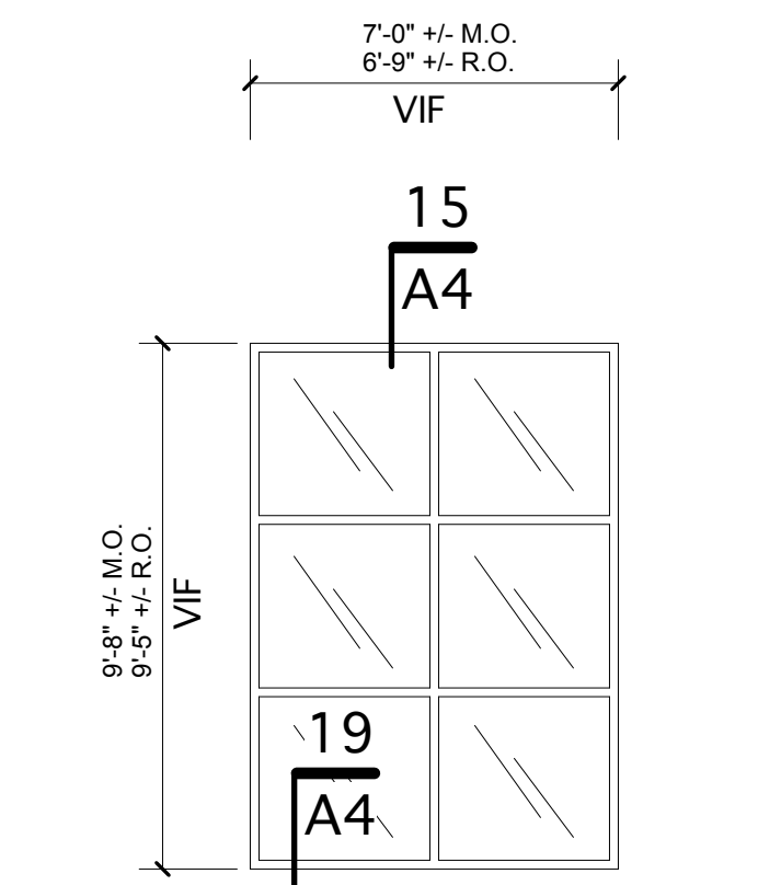
16 FIXED FRAME UNIT 16 Units Req'd
