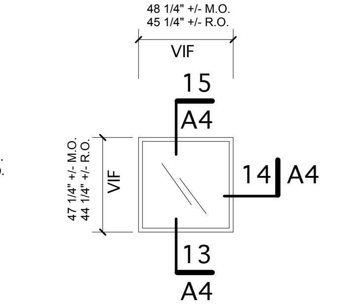
1 FIXED FRAME UNIT 13 Units Req'd
