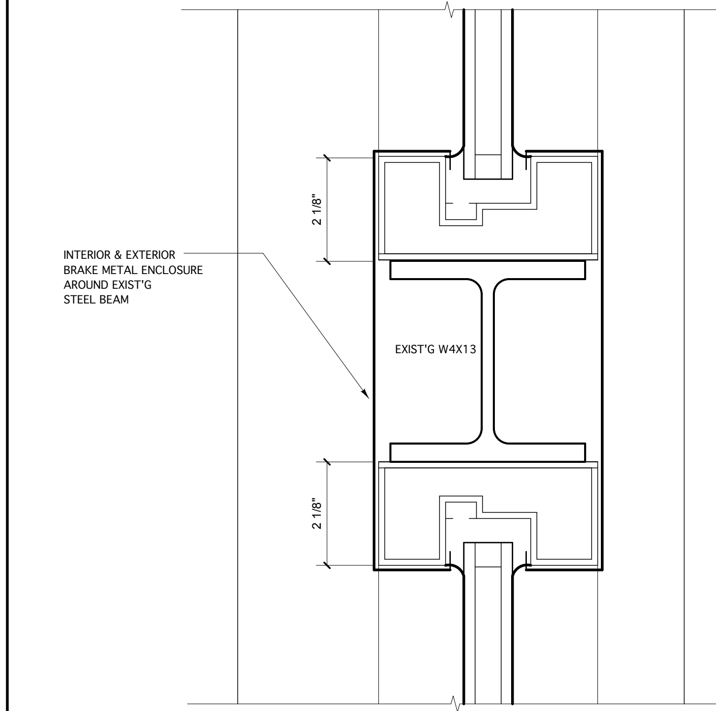
19 WINDOW HORIZONTAL MULLION DETAIL 6"=1'-0"
