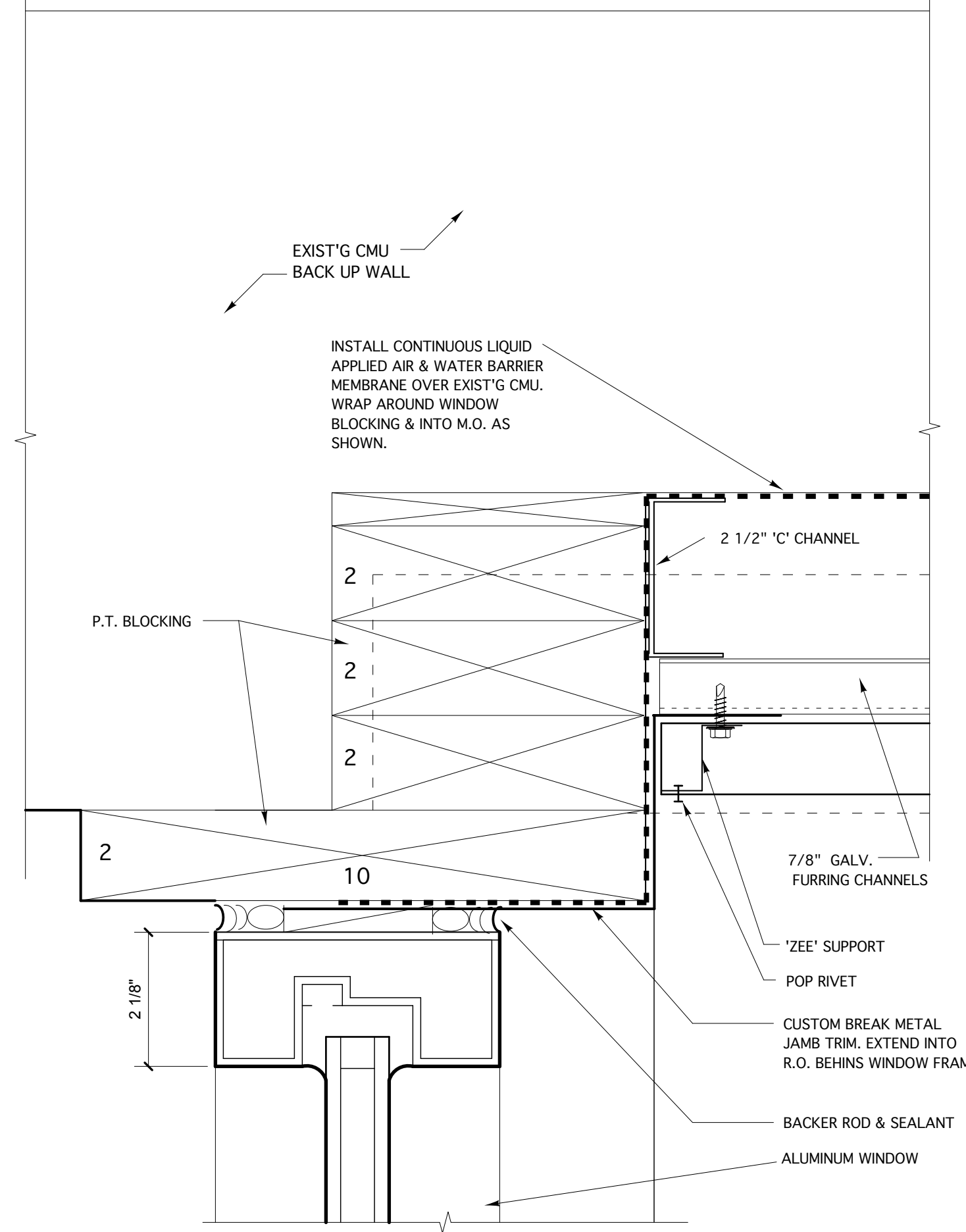
17 WINDOW JAMB DETAIL 6"=1'-0"
