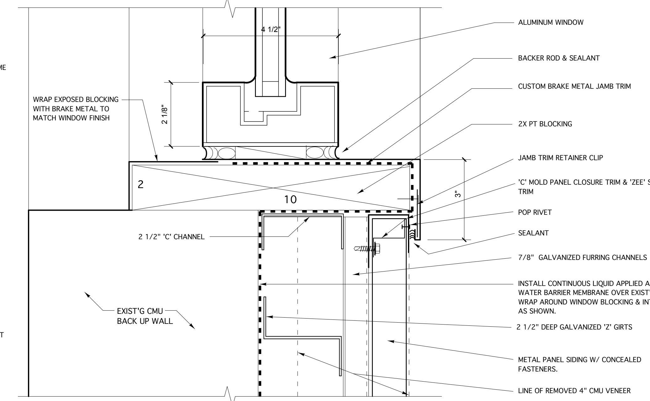
14 WINDOW JAMB DETAIL 6"=1'-0"
