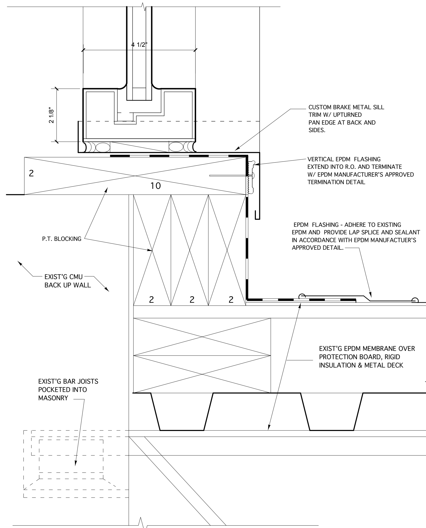
18 WINDOW SILL DETAIL 6"=1'-0"
