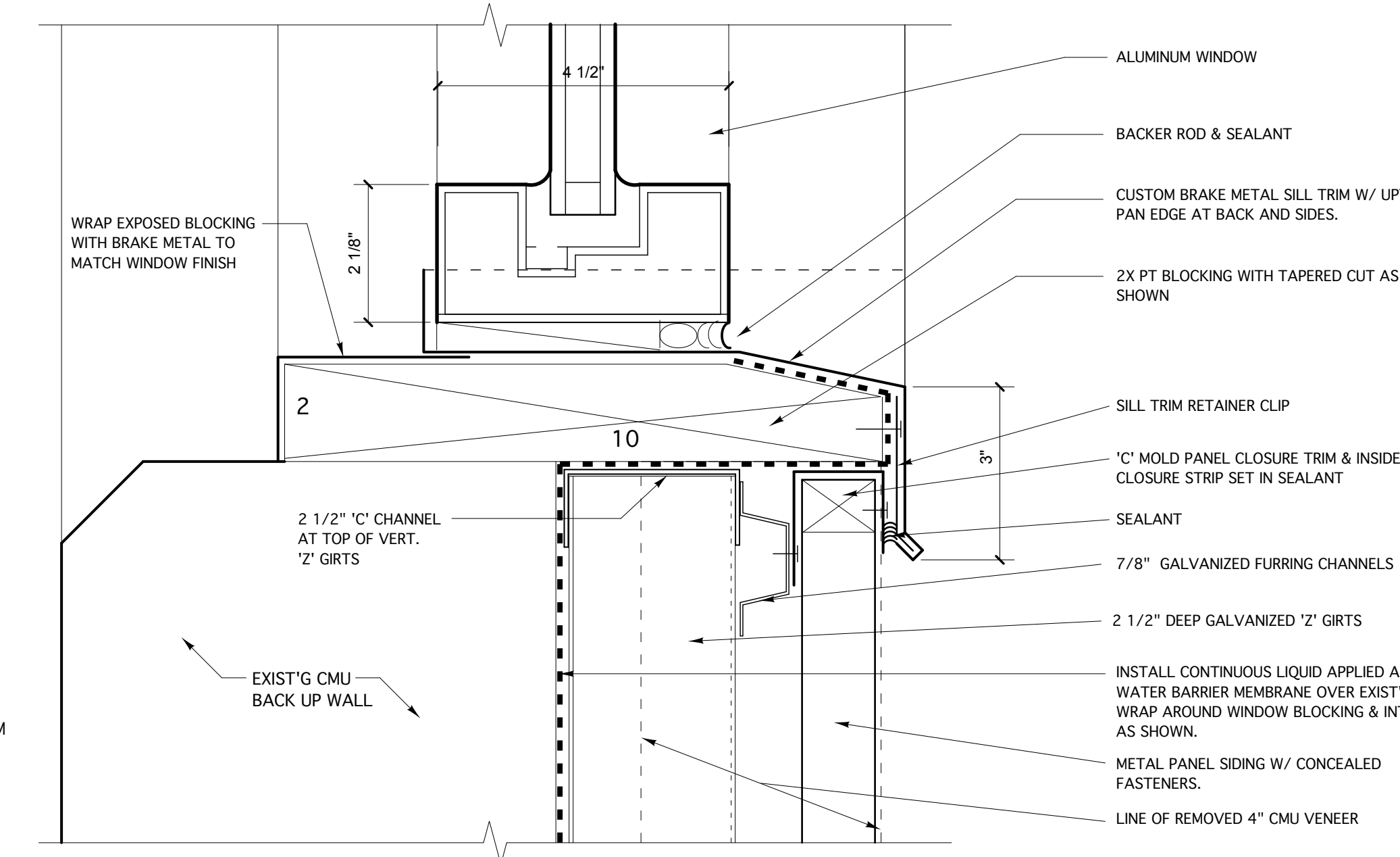
13 WINDOW SILL DETAIL 6"=1'-0"
