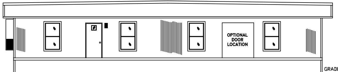
RIGHT SIDE WALL ELEVATION
