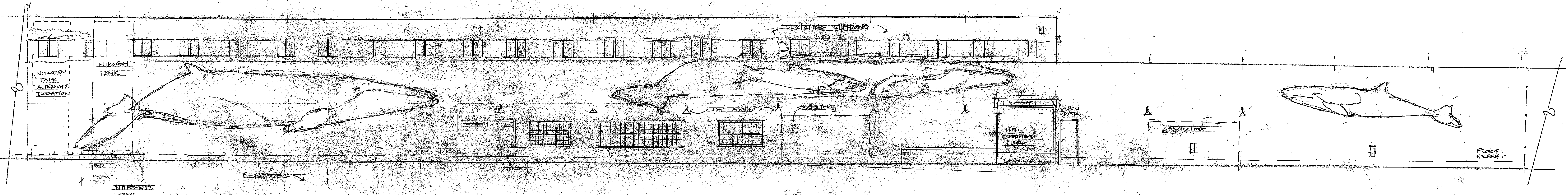
MAINE STATE PIER EAST ELEVATION SCALE 1/8" = 1'-0" 0 10 20
