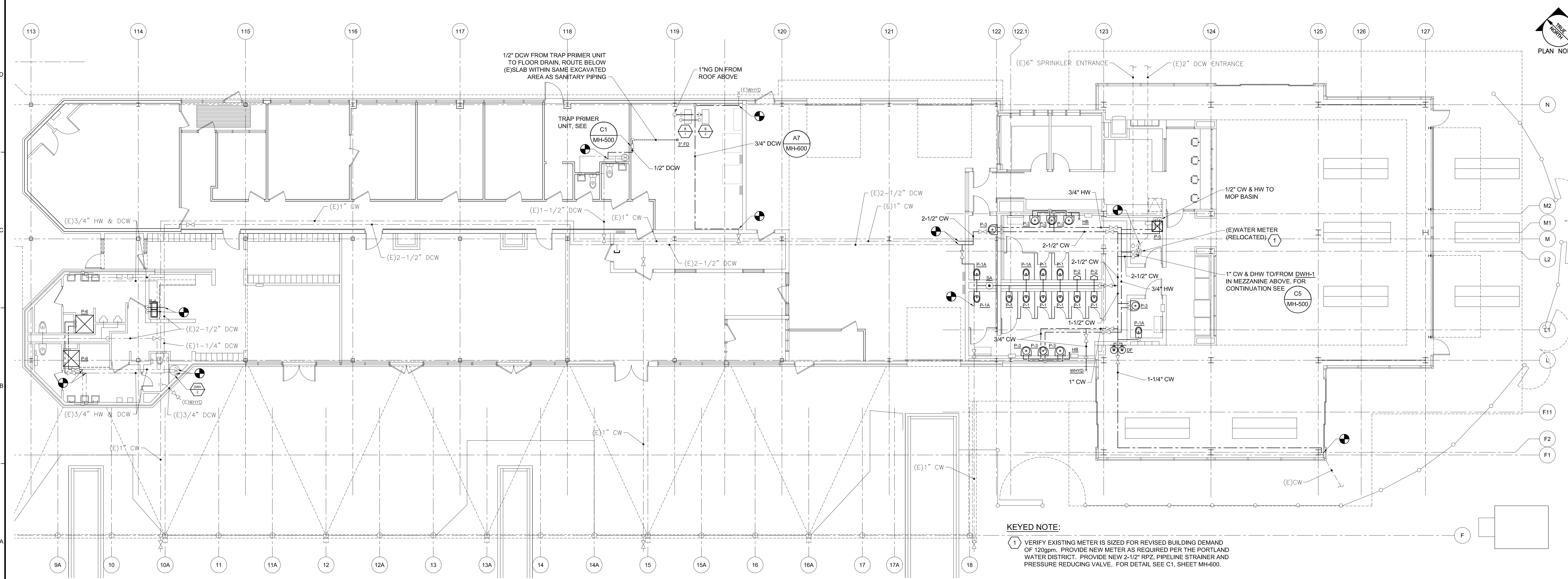
A1 DOMESTIC PIPING PLAN 1/8" = 1'-0"
