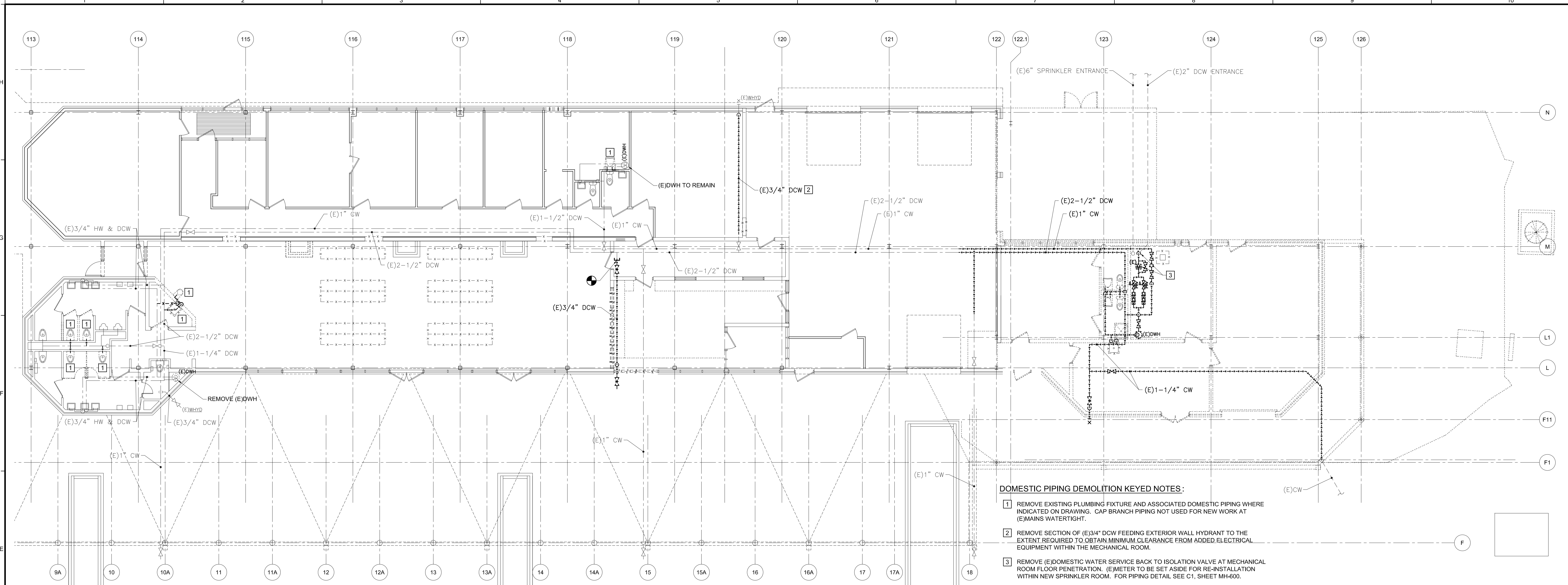
E1 DOMESTIC PIPING DEMOLITION PLAN 1/8" = 1'-0"
