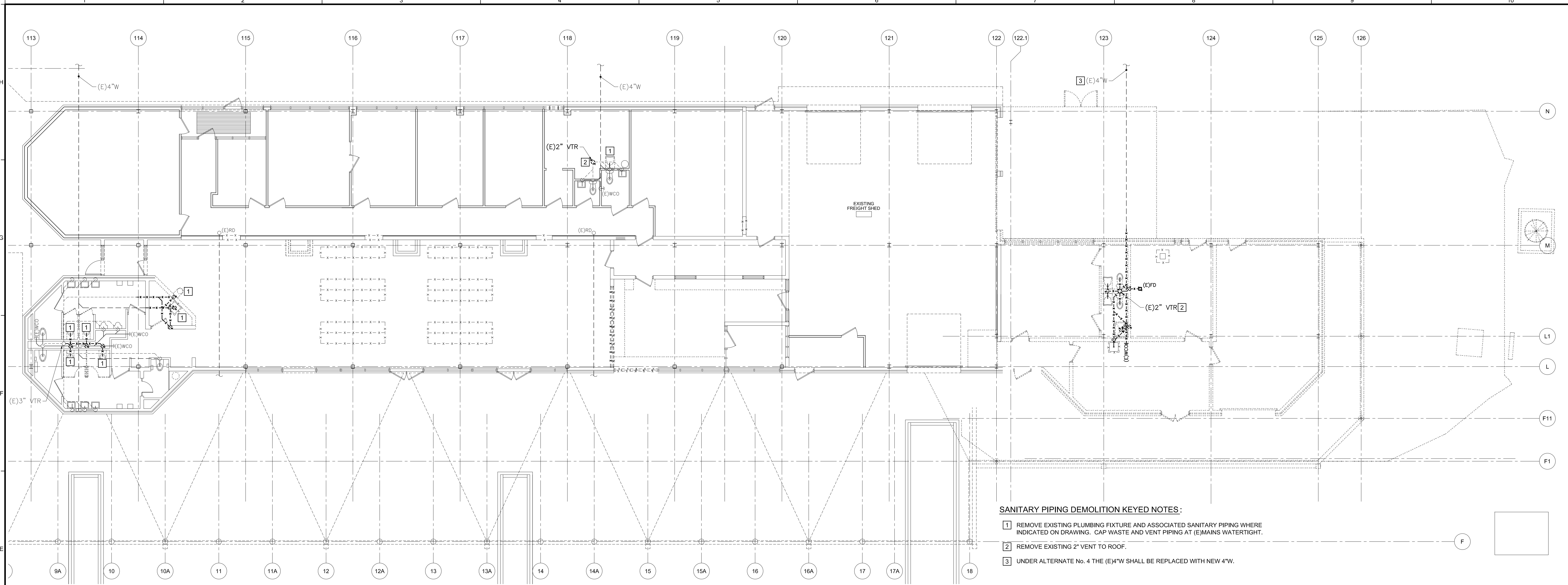
E1 SANITARY PIPING DEMOLITION PLAN 1/8" = 1'-0"
