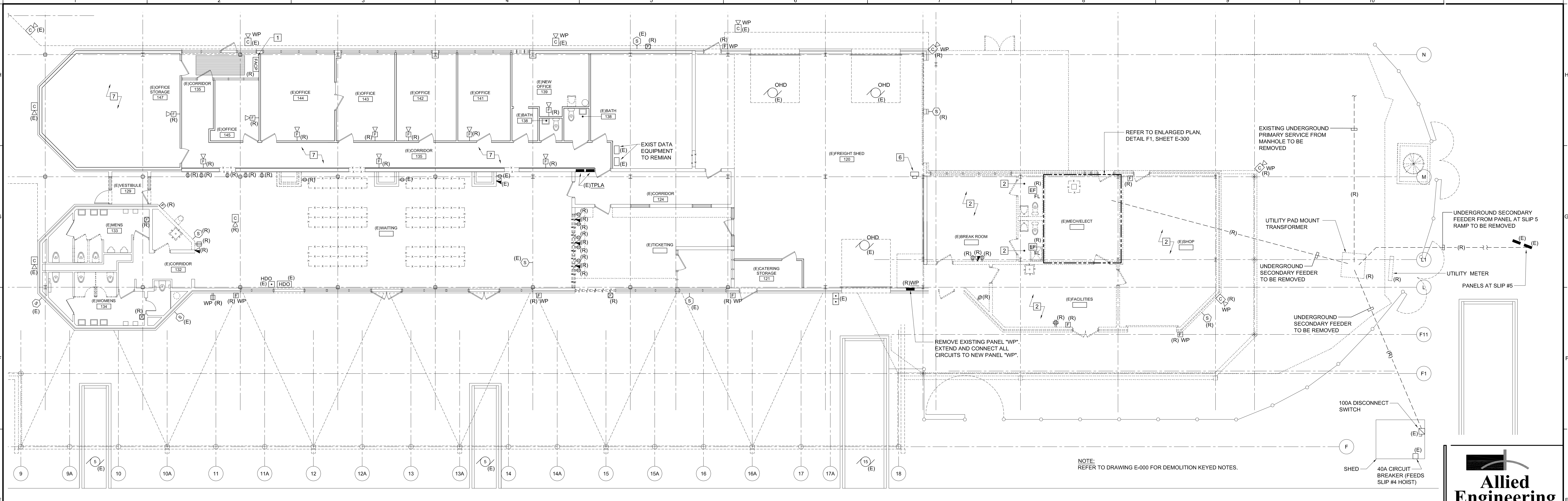
E1 ELECTRICAL POWER DEMOLITION PLAN
