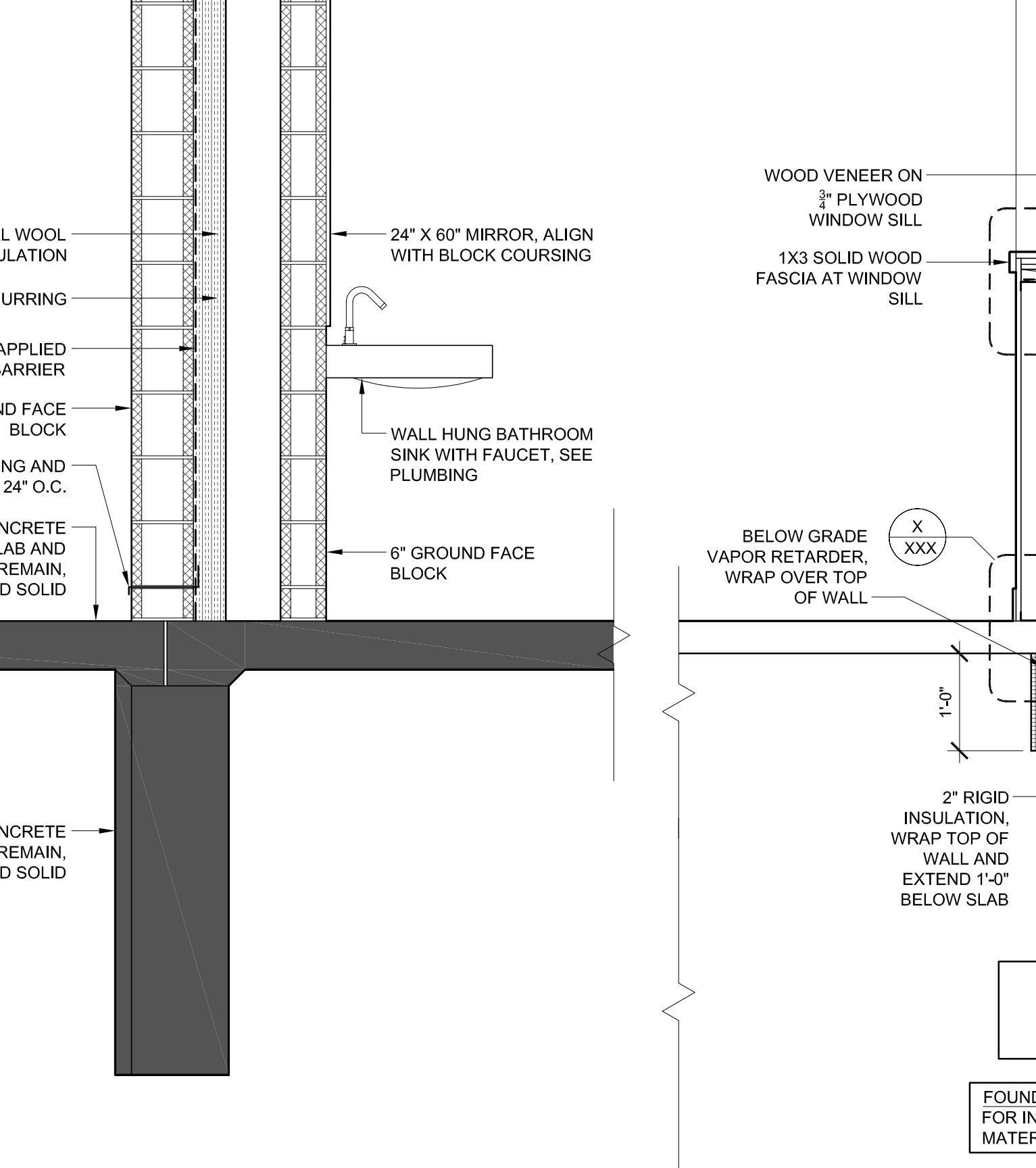
6 WALL SECTION AT OFFICE WALL SCALE: 3/4" = 1'-0"
