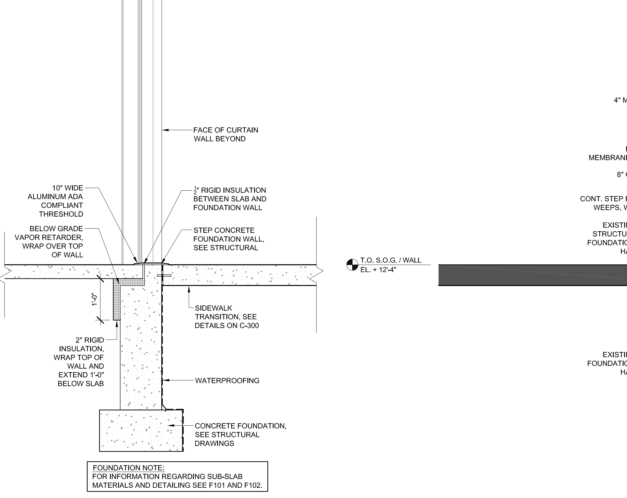
4 WALL SECTION AT BI-FOLD DOOR SCALE: 3/4" = 1'-0"
