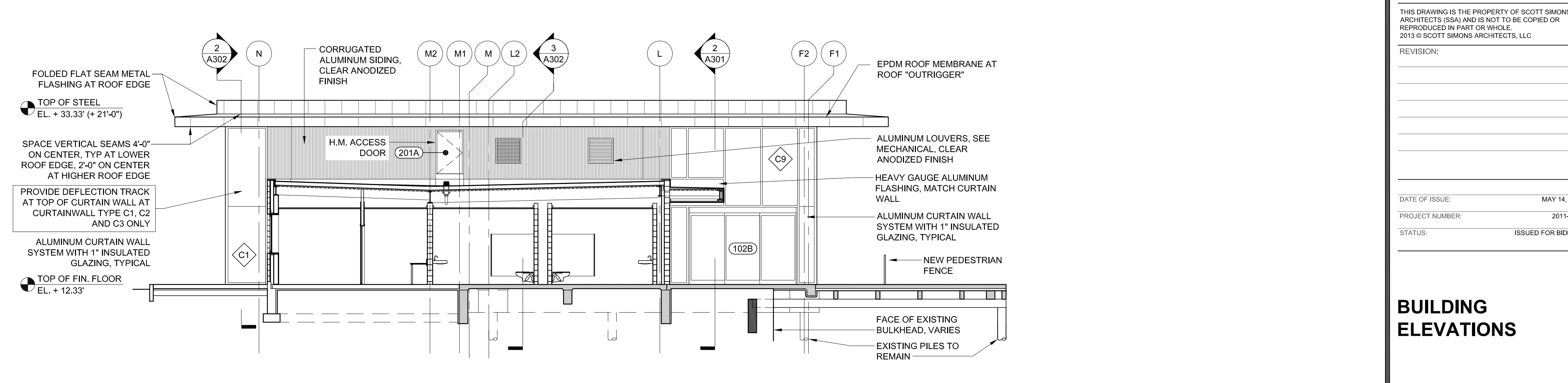
5 NORTH BUILDING ELEVATION/SECTION SCALE: 1/8" = 1'-0"
