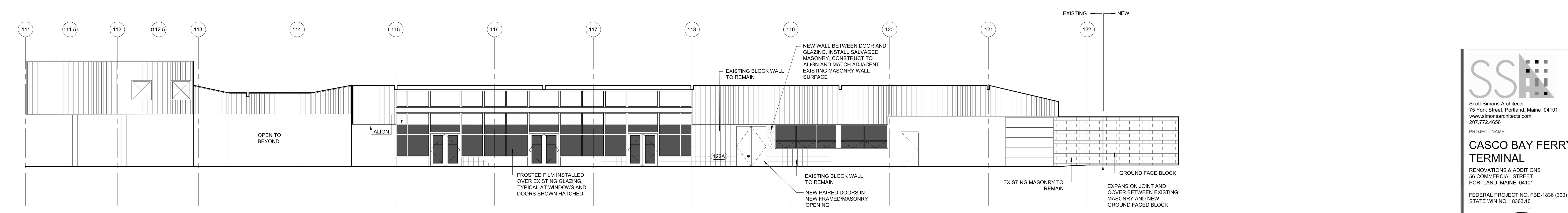
3 BUILDING ELEVATION/UNDER CANOPY SCALE: 1/8" = 1'-0"
