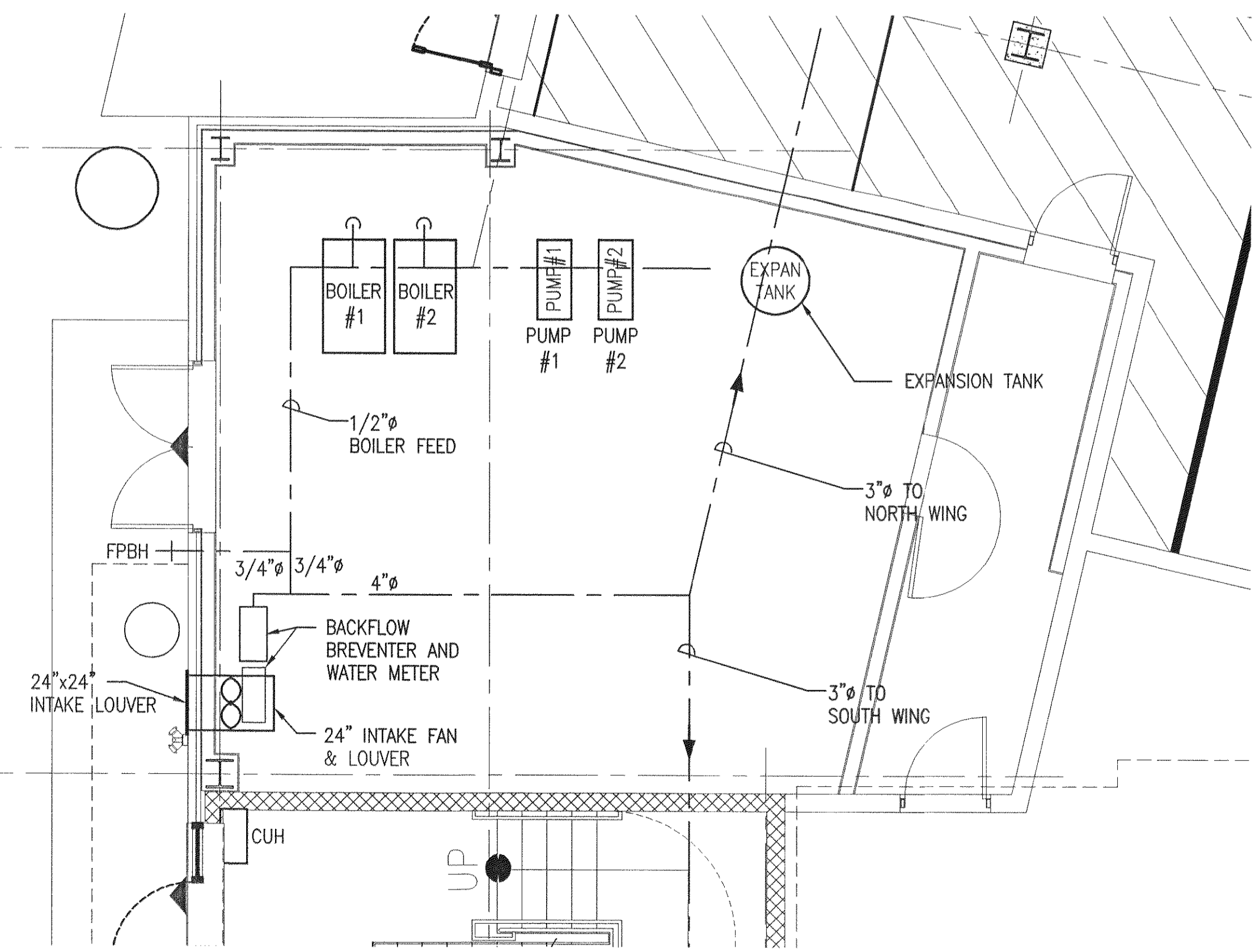
BOILER ROOM PLAN COLD WATER SCALE: 1/4"=1'-0"
