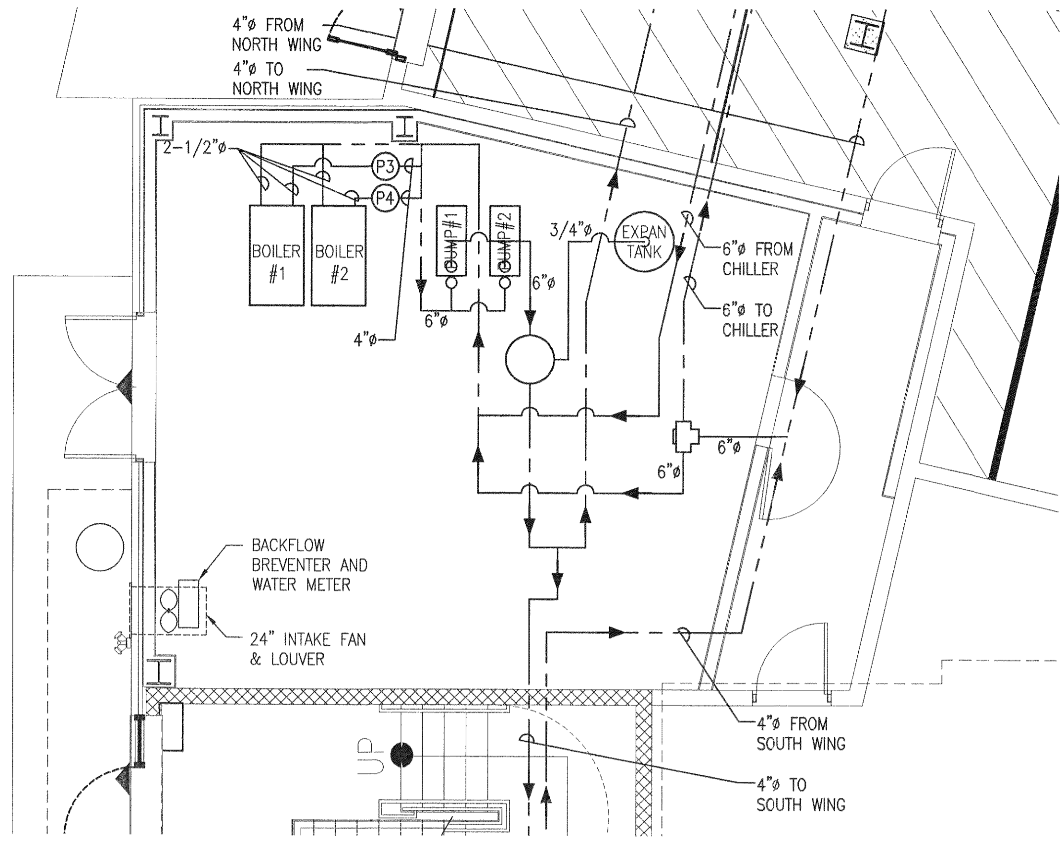
BOILER ROOM PLAN HYDRONIC PIPING SCALE: 1/4"=1'-0"
