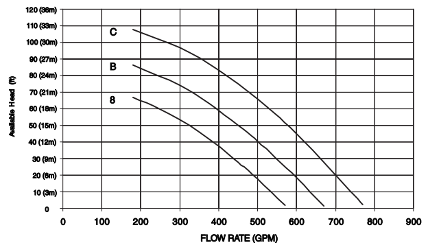
Fig. 46 — 30RB160, 170, 190 — Single Pump Envelope Curves
