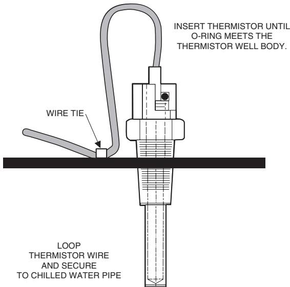
Fig. 50 — Dual Leaving Water Thermistor (Part No. 00PPG00008105A)
