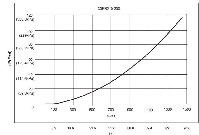
Fig. 38 — 30RB210-300 Cooler Pressure Drop Curve
