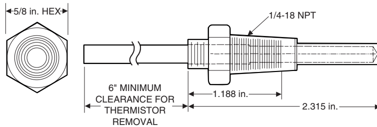
Fig. 49 — Dual Leaving Water Thermistor Well (Part No. 00PPG00008100A)
