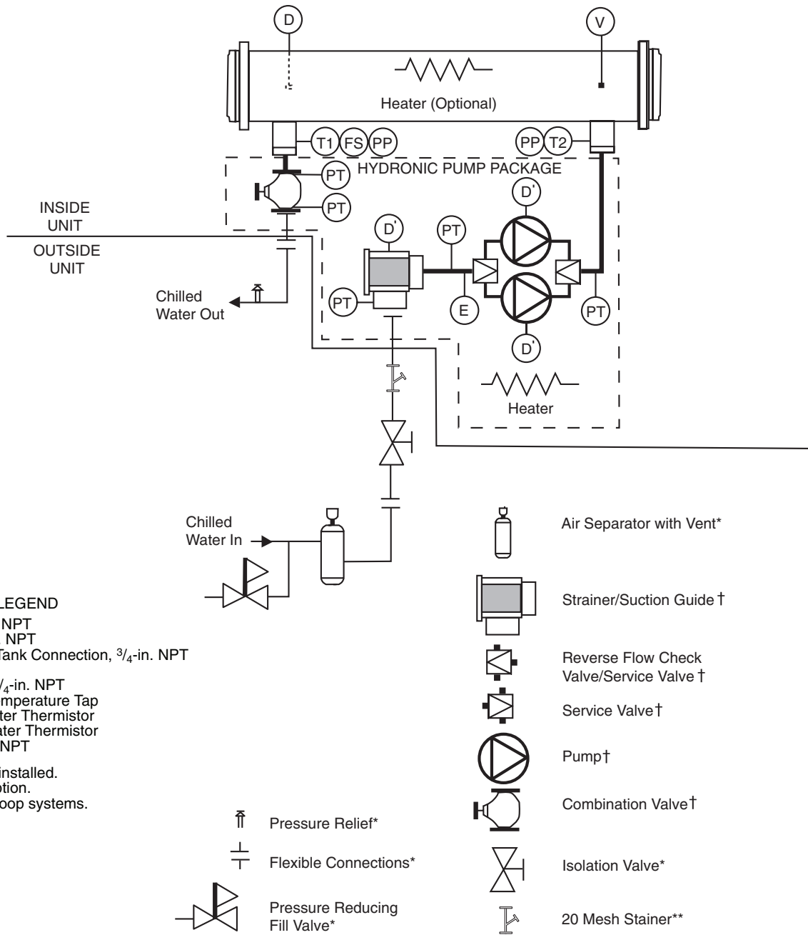
Fig. 21 — Typical Piping Diagram on 30RB Units with Hydronic Package — Dual Pumps
