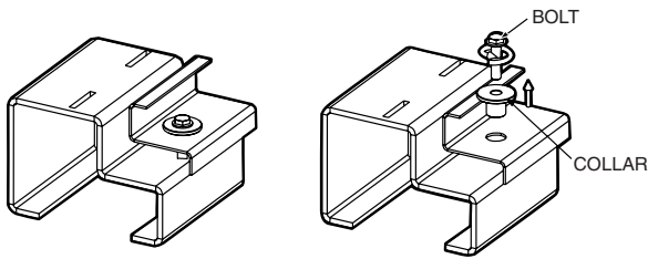
Fig. 19 — Compressor Rack Holddown Bolts
