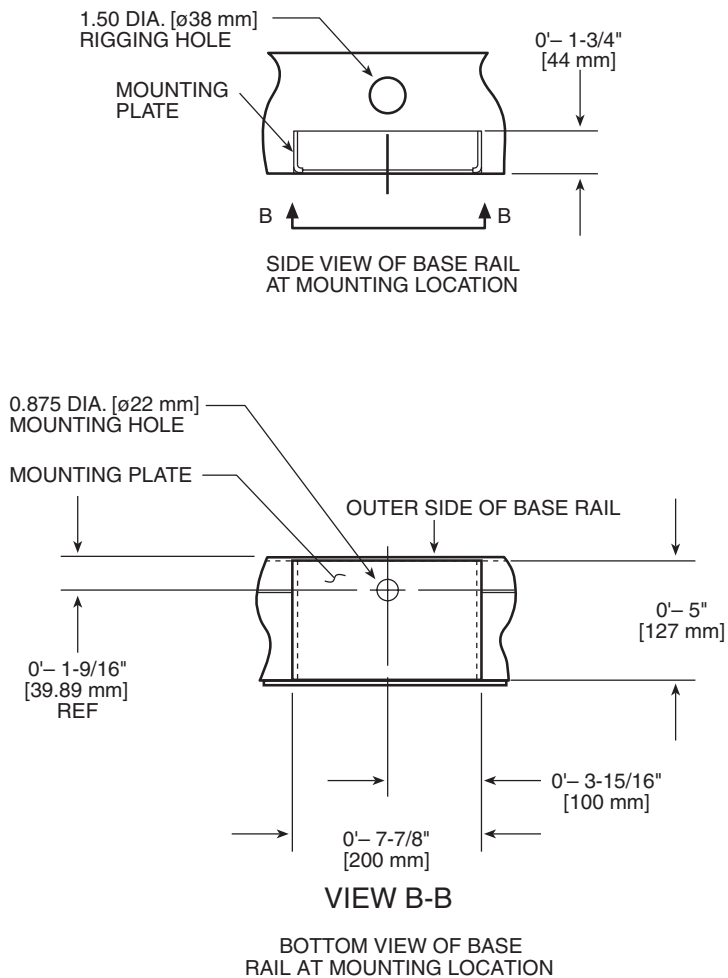
Fig. 16 — 30RB Mounting Plate
