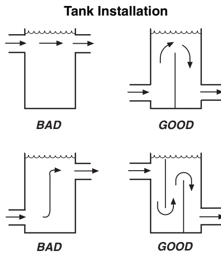
Fig. 24 — Tank Baffling
