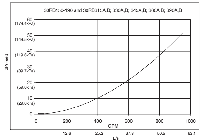
Fig. 37 — 30RB150-190 and 30RB315A,B; 345A,B; 360A,B; 390A,B Cooler Pressure Drop Curve
