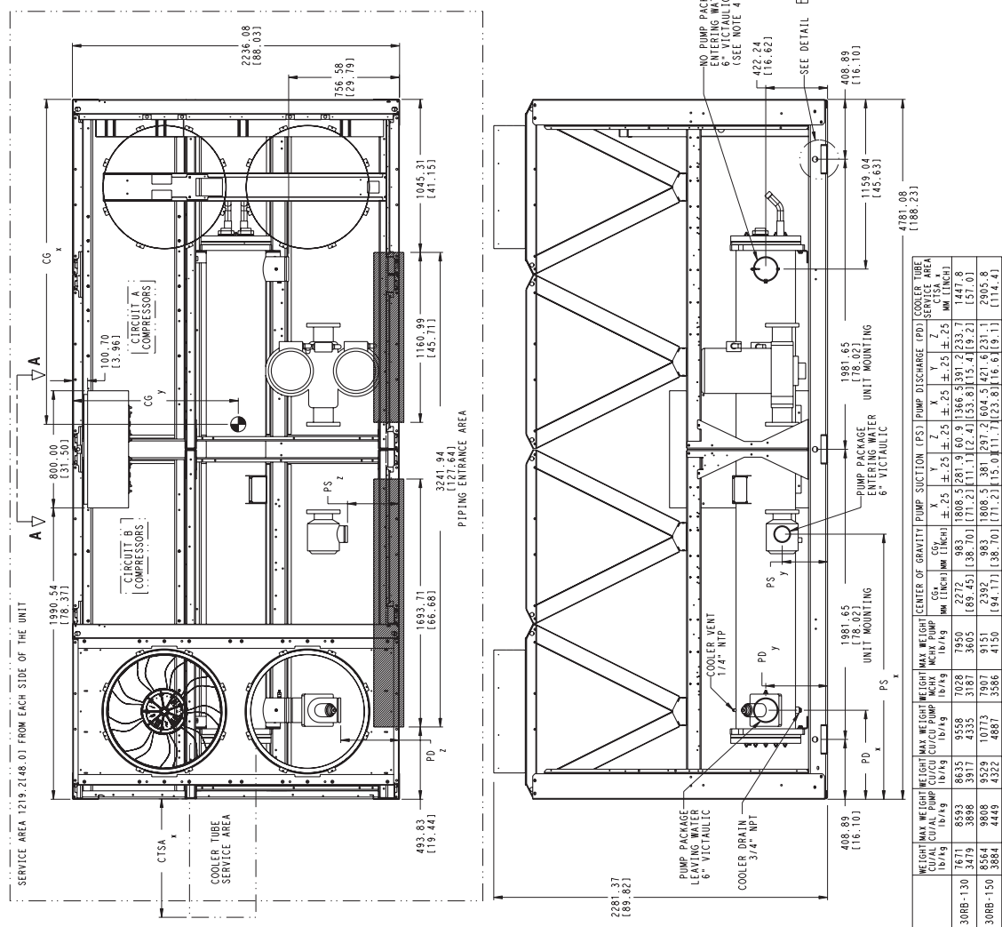
Fig. 7 — 30RB130, 150 Air-Cooled Chiller Dimensions
