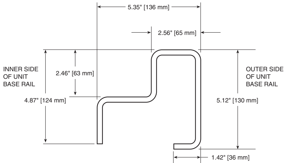
Fig. 15 — 30RB Base Rail Cross Section
