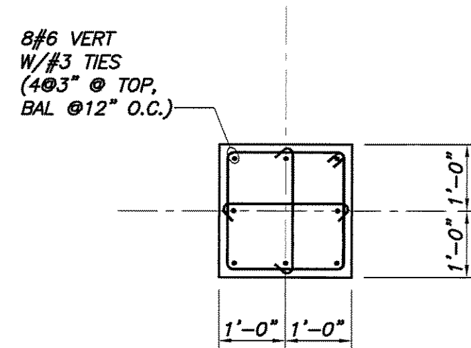
PIER P2 DETAIL
