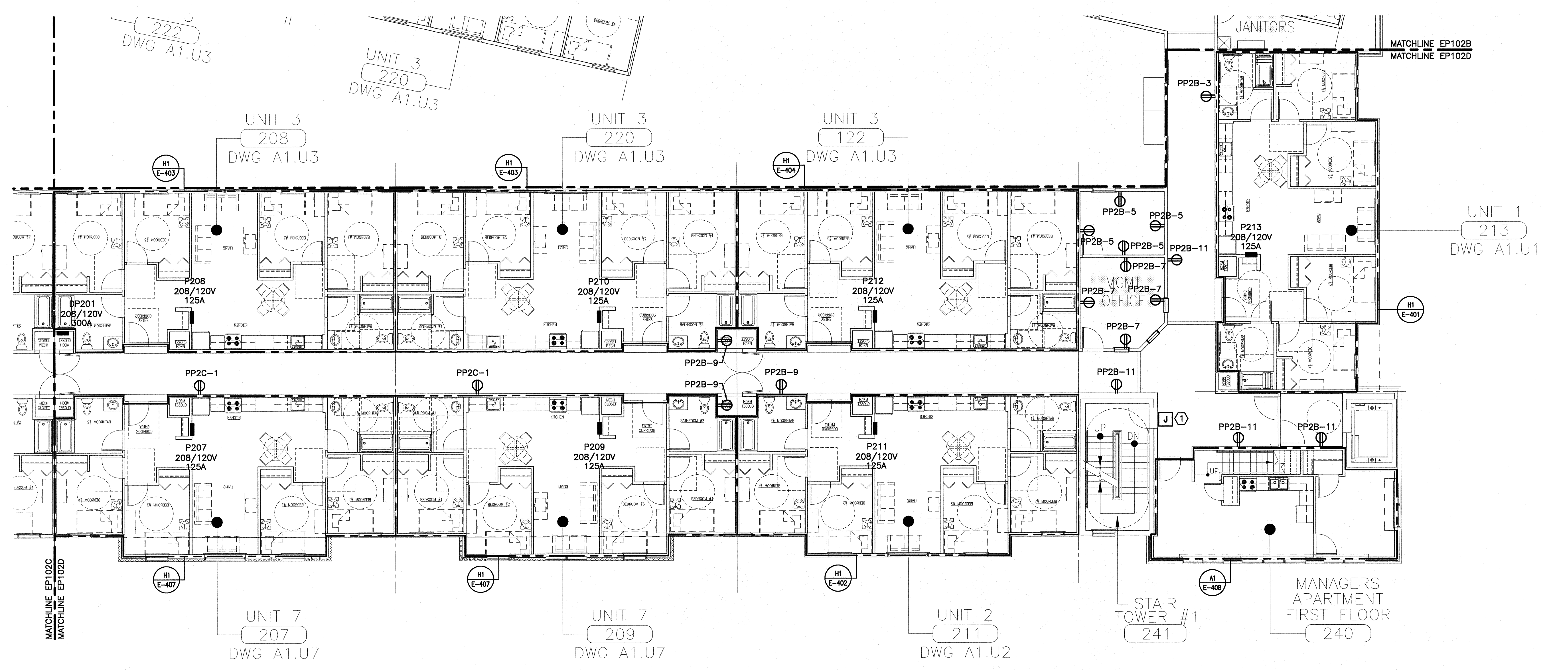
A1 SECOND FLOOR PLAN
