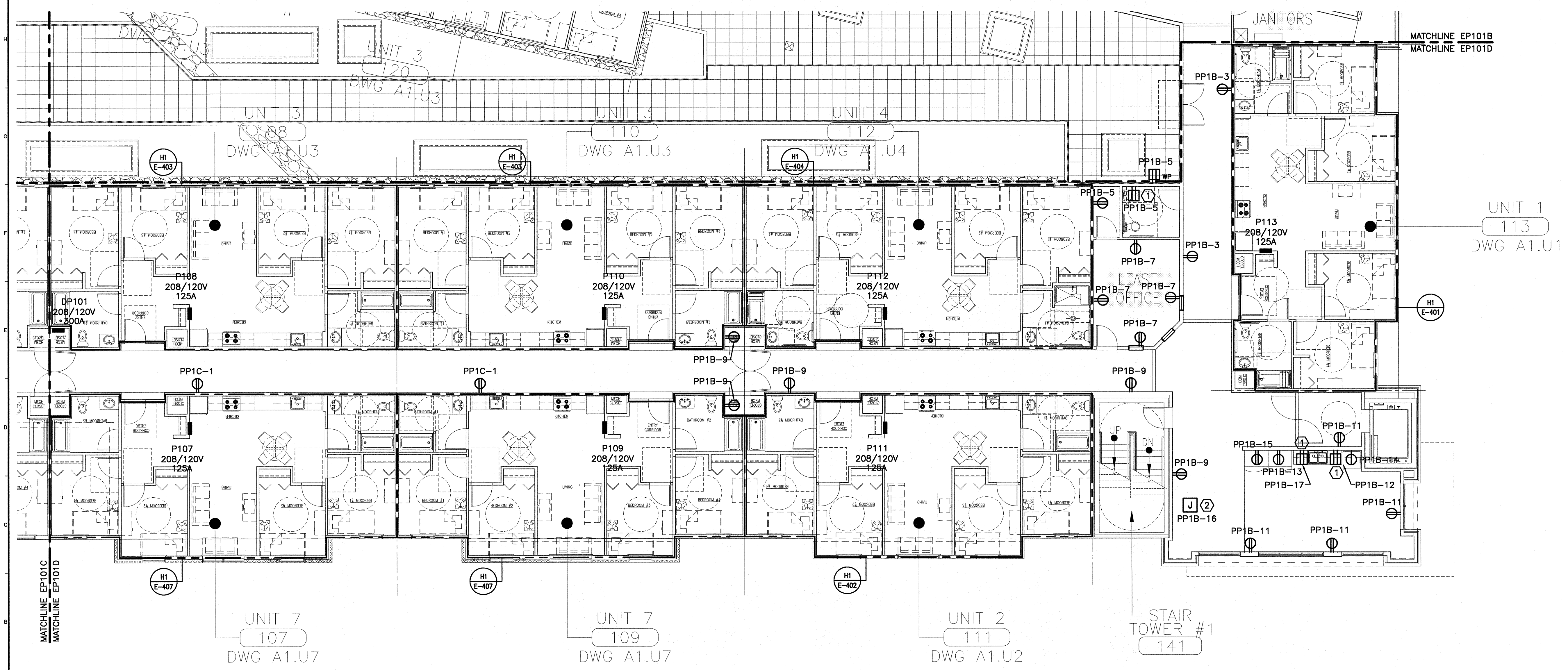
A1 FIRST FLOOR PLAN
