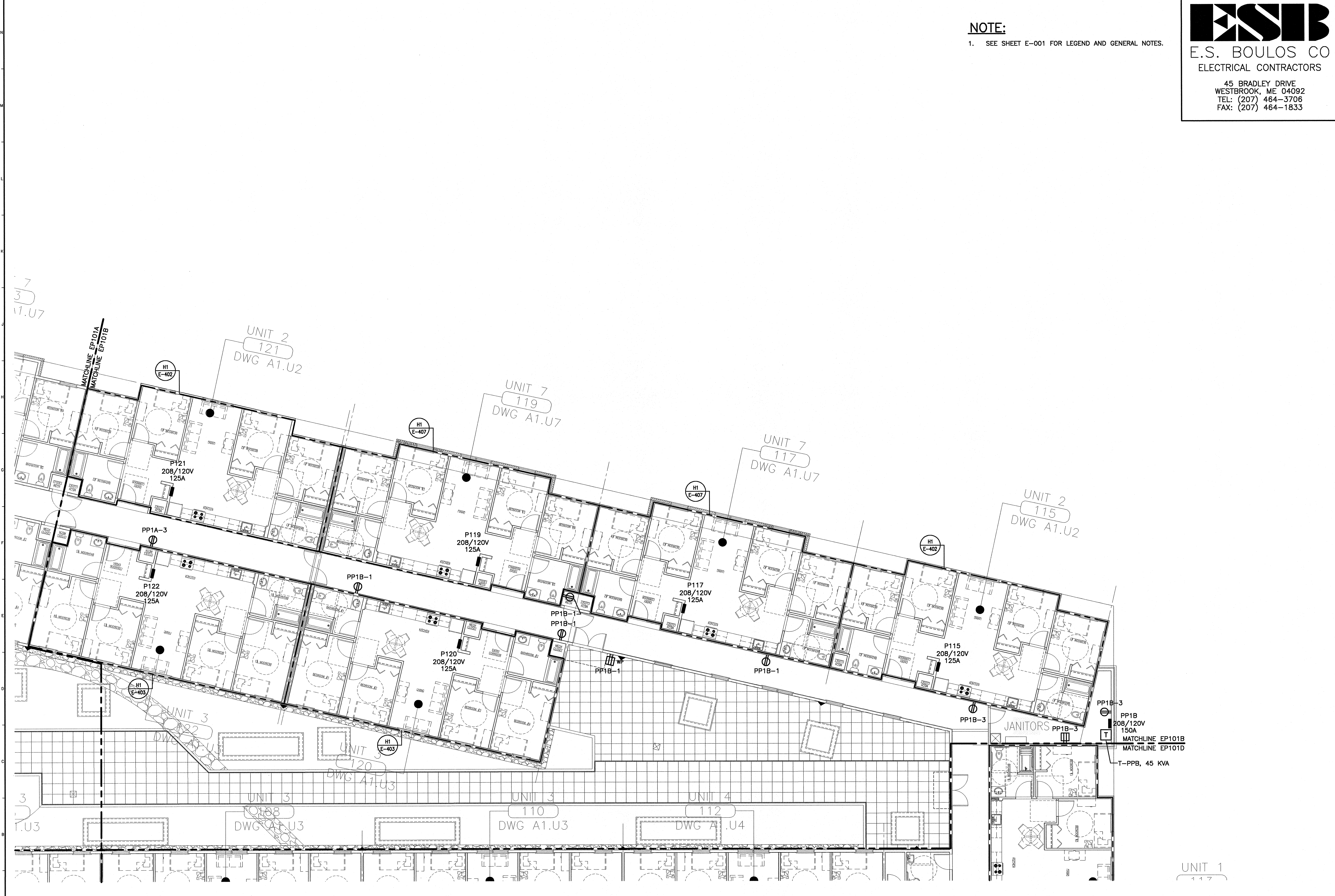
A1 FIRST FLOOR PLAN
