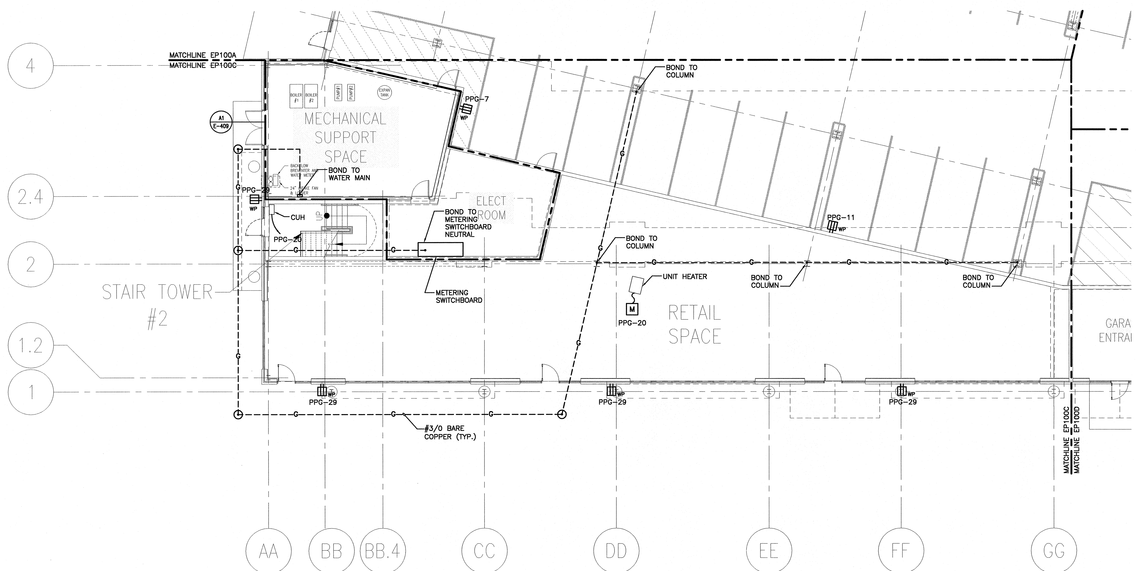
A1 LOWER LEVEL PLAN 1/8"=1'-0"
