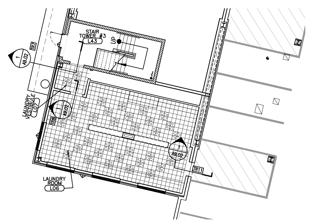
1 FLOOR FINISH & PATTERN PLAN LOWER LEVEL REFERENCED FROM: SCALE: 3/32" = 1'-0"
