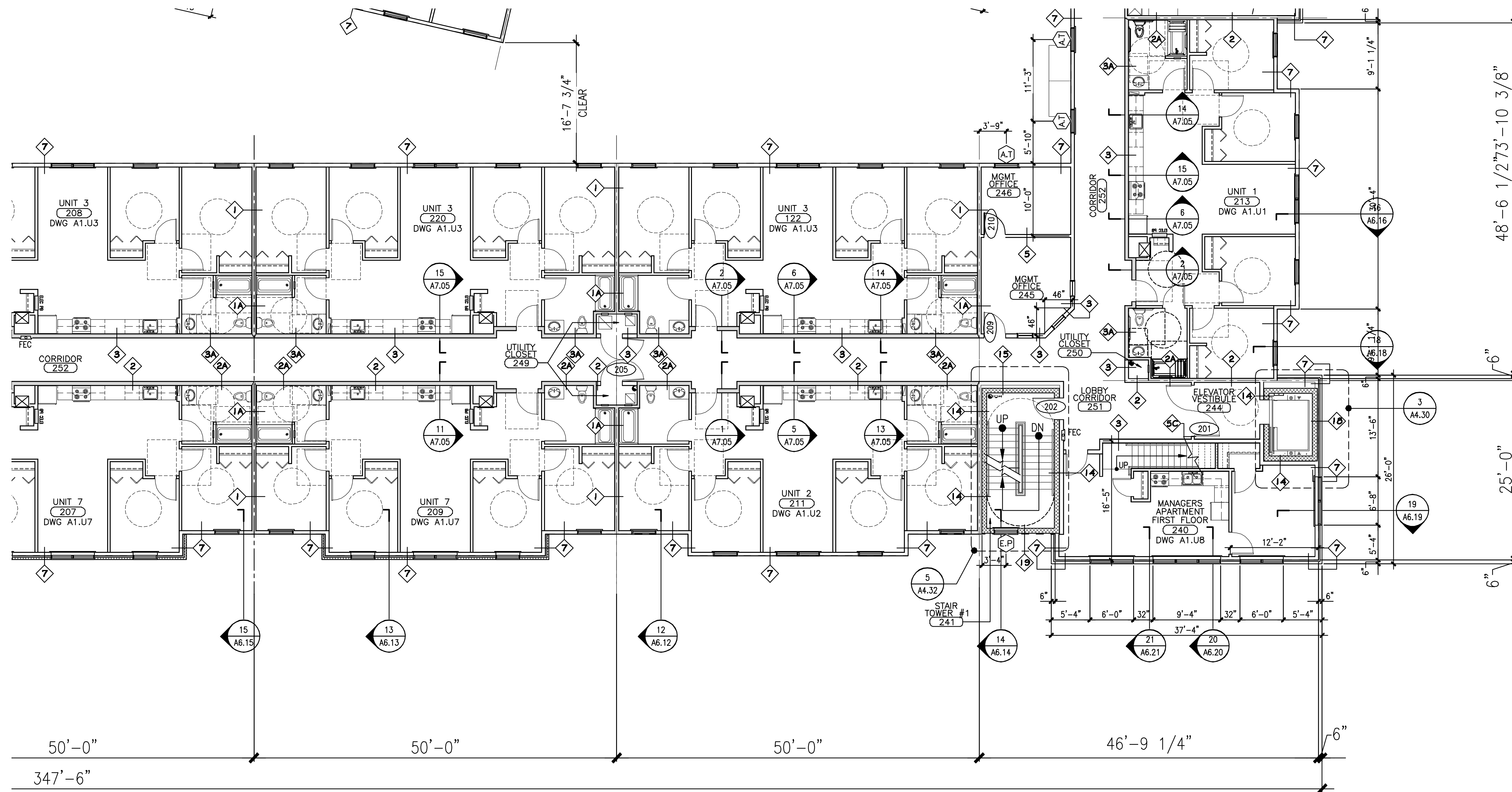
D ENLARGED PLAN - SECOND FLOOR - AREA D REFERENCED FROM: SCALE: 1/4" = 1'-0"
