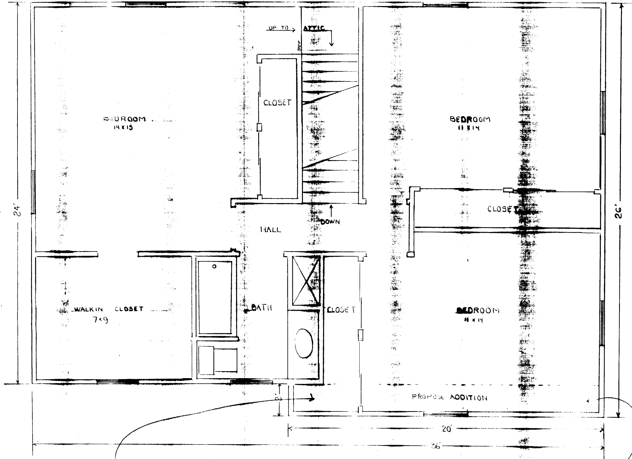
AMENDED SECOND FLOOR DETAIL WITH ADDITIONAL 2'x20' CANTILEVER OVER ENTRY
