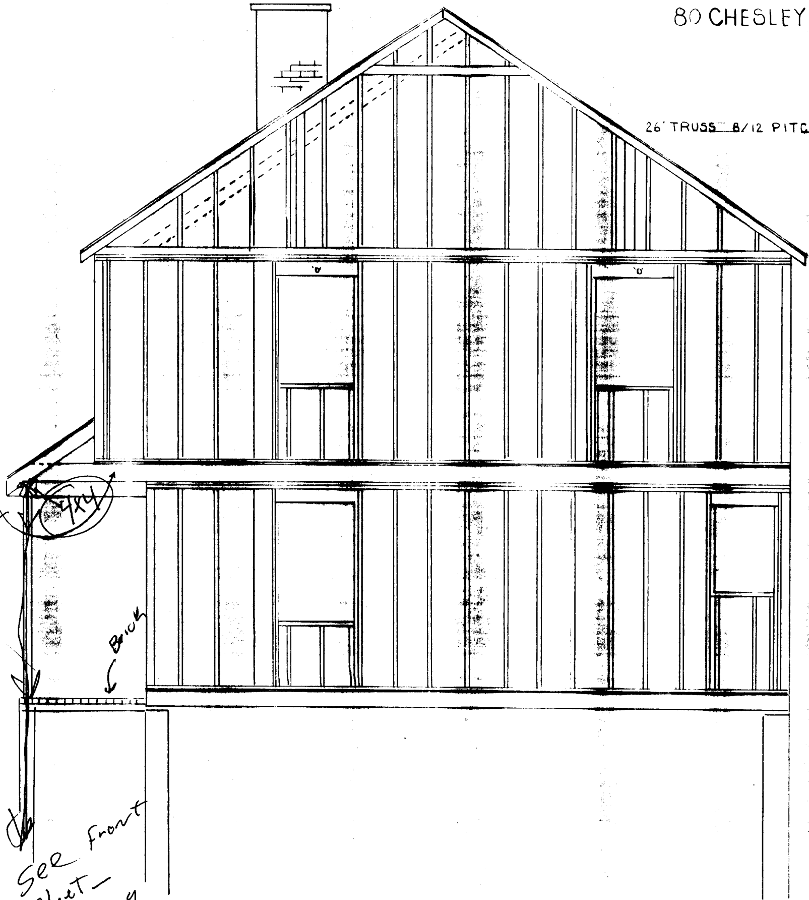
AMENDED RIGHT ELEVATION FRAMING DETAIL
