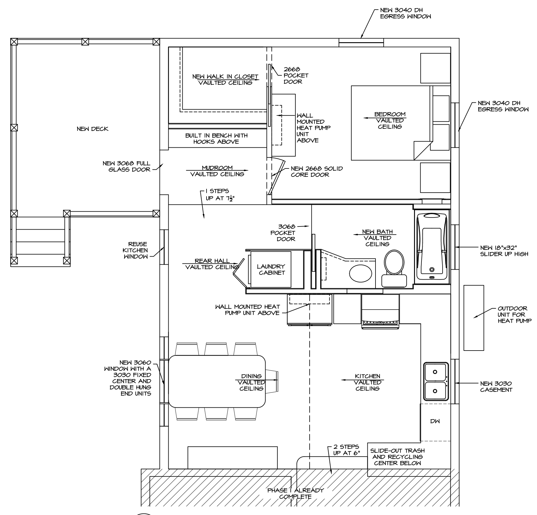
1 PROPOSED LAYOUT SCALE: 1/4" = 1'-0"
