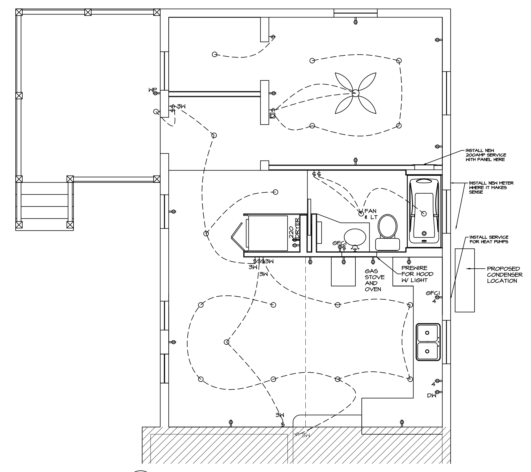
3 PROPOSED ELECTRICAL LAYOUT SCALE: 1/4" = 1'-0"
