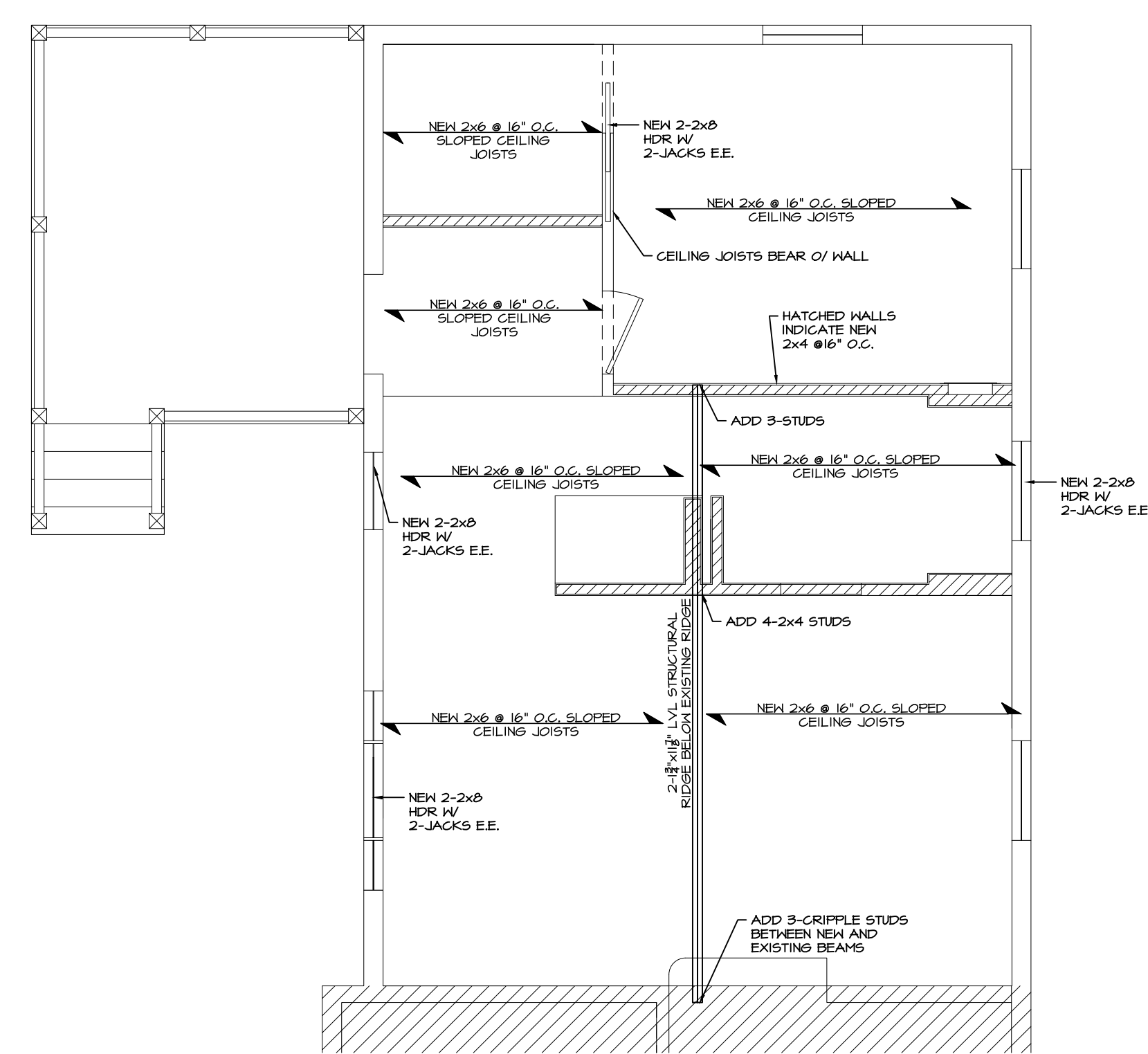
5 FIRST FLOOR CEILING FRAMING PLAN SCALE: 1/2" = 1'-0"
