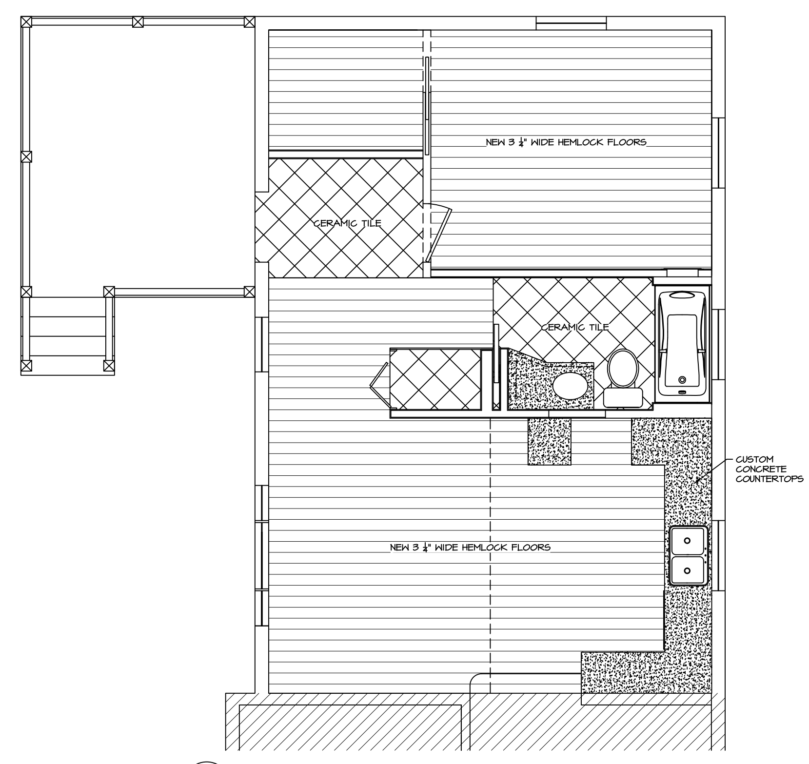
2 FINISH SCHEDULE SCALE: 1/4" = 1'-0"
