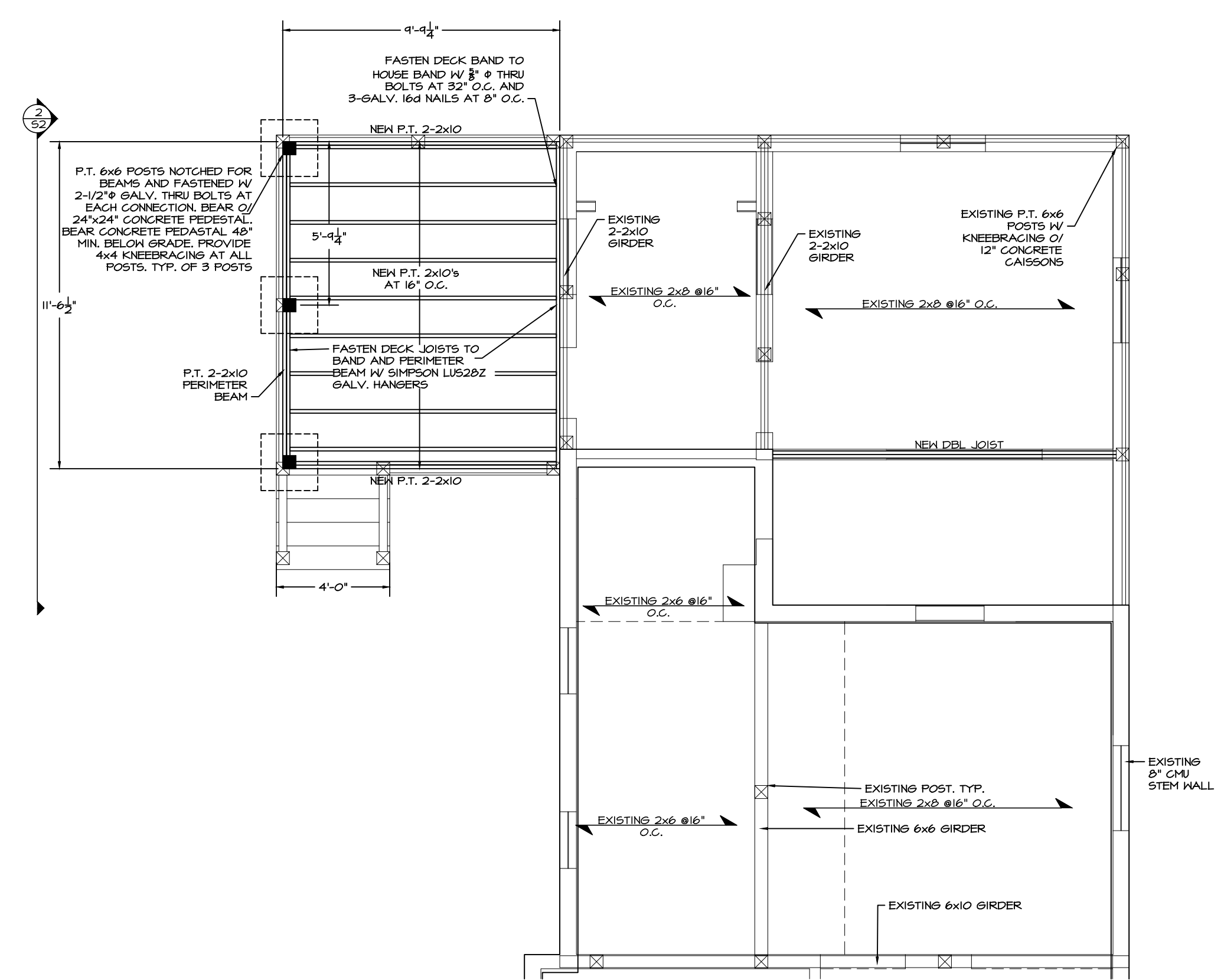
4 FIRST FLOOR FRAMING REINF. PLAN SCALE: 1/2" = 1'-0"
