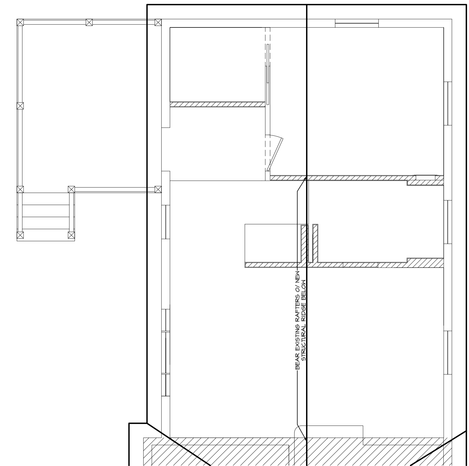
6 ROOF PLAN SCALE: 1/4" = 1'-0"
