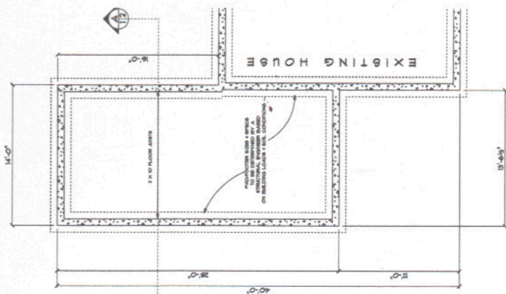
FOUNDATION SCALE: 1/4" = 1'-0"
