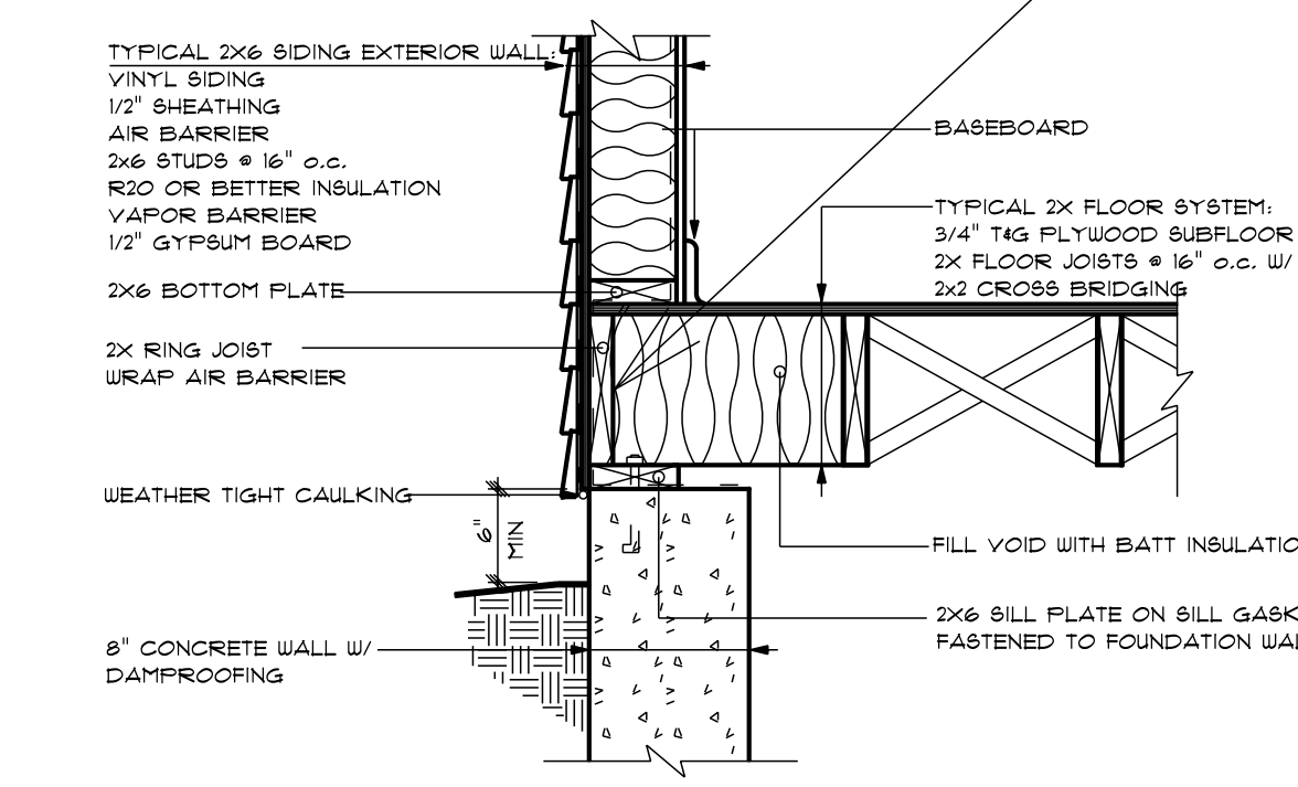
2X6/SIDING WALL AT FOUNDATION
