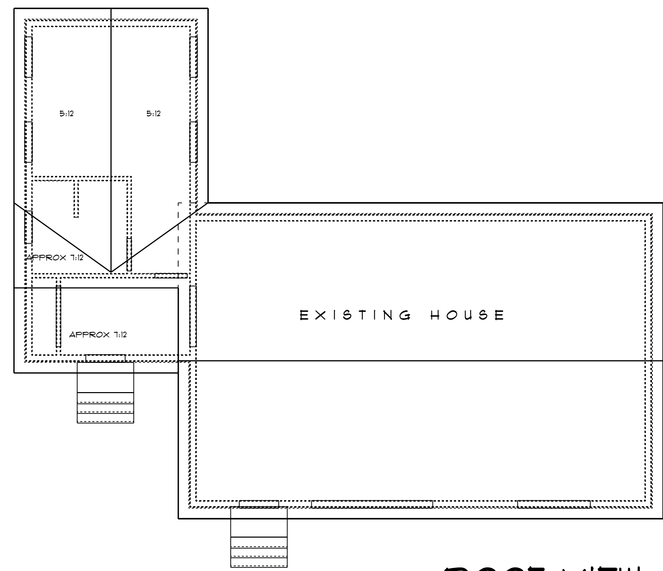
ROOF VIEW SCALE: 1/8" = 1'-0"
