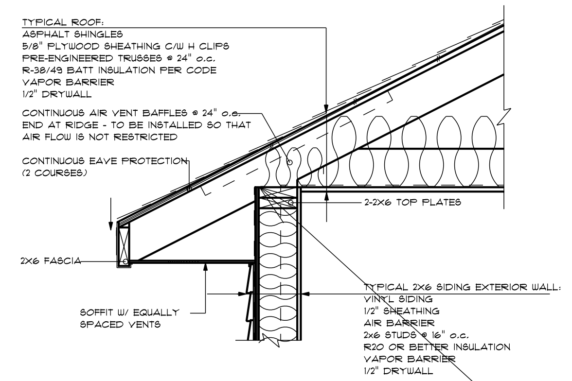
2X6/SIDING EAVE
