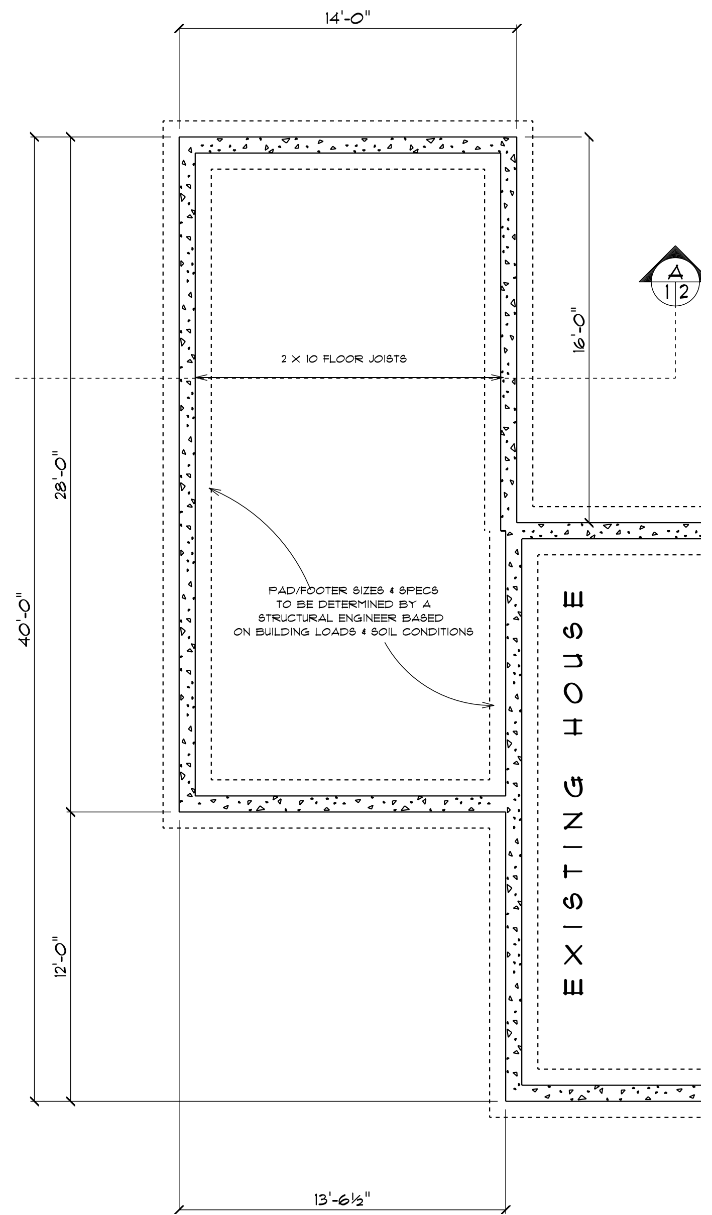
FOUNDATION SCALE: 1/4" = 1'-0"
