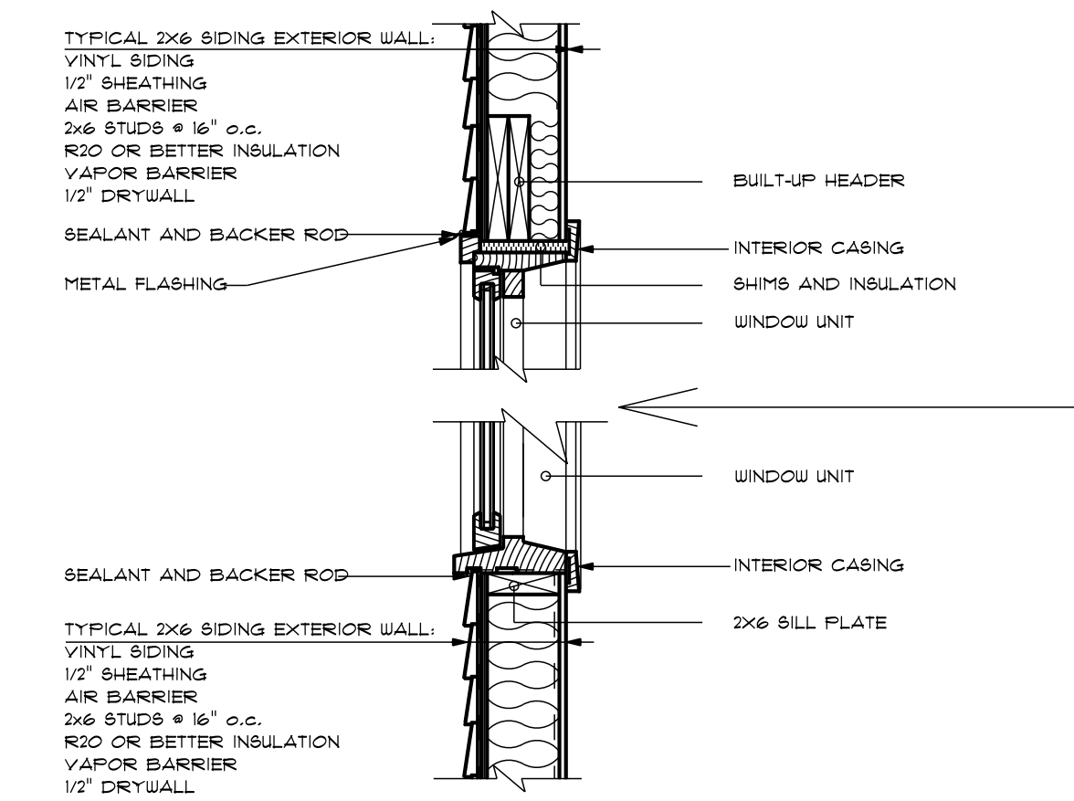
2X6/SIDING HEADER & BILL
