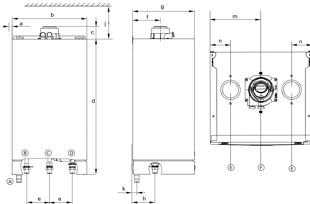
Fig. 1 Front view
