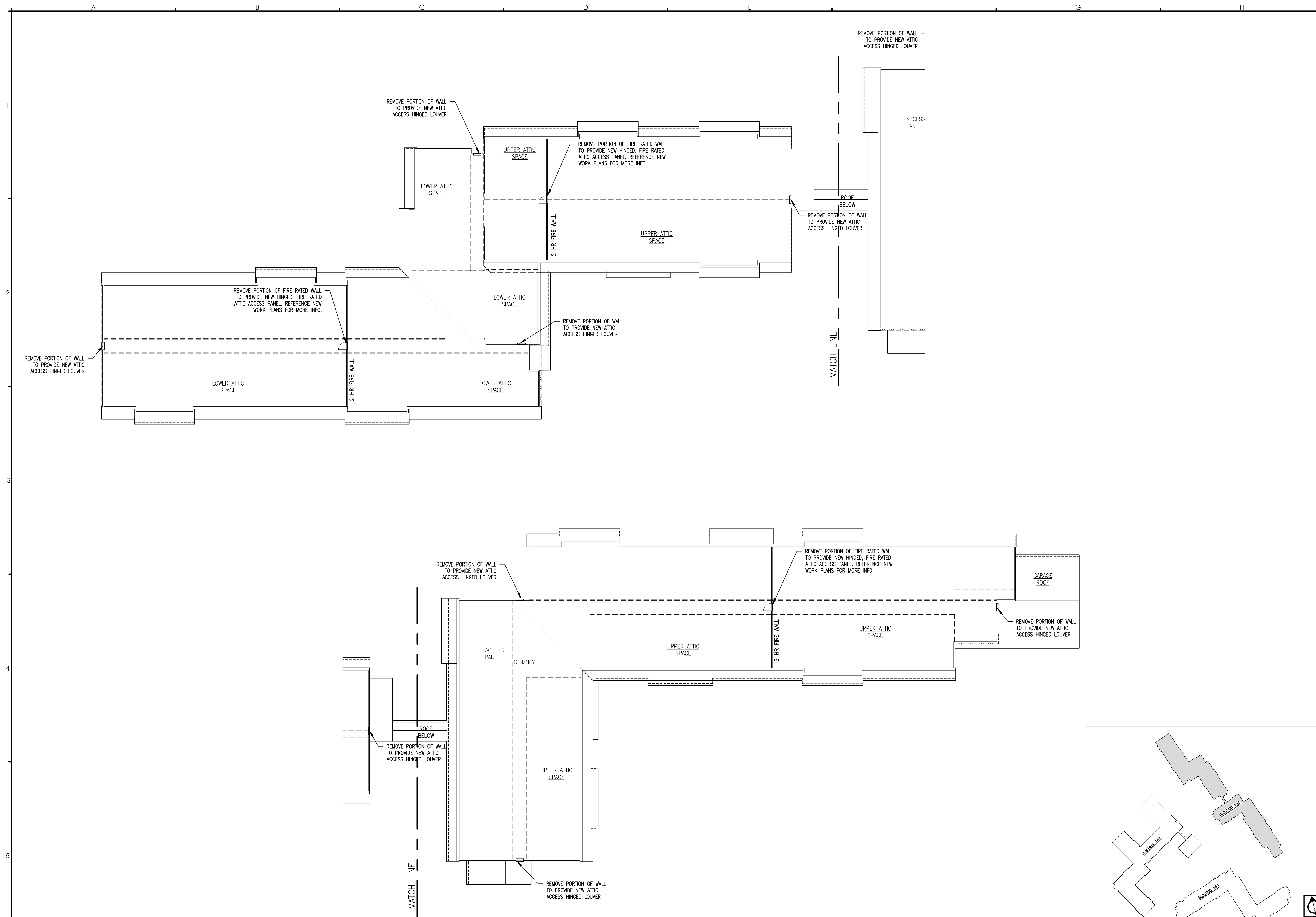
A5 BUILDING NO. 151 - ATTIC REMOVALS PLAN REFERENCED FROM: TP2 SCALE: 1/16" = 1'-0"
