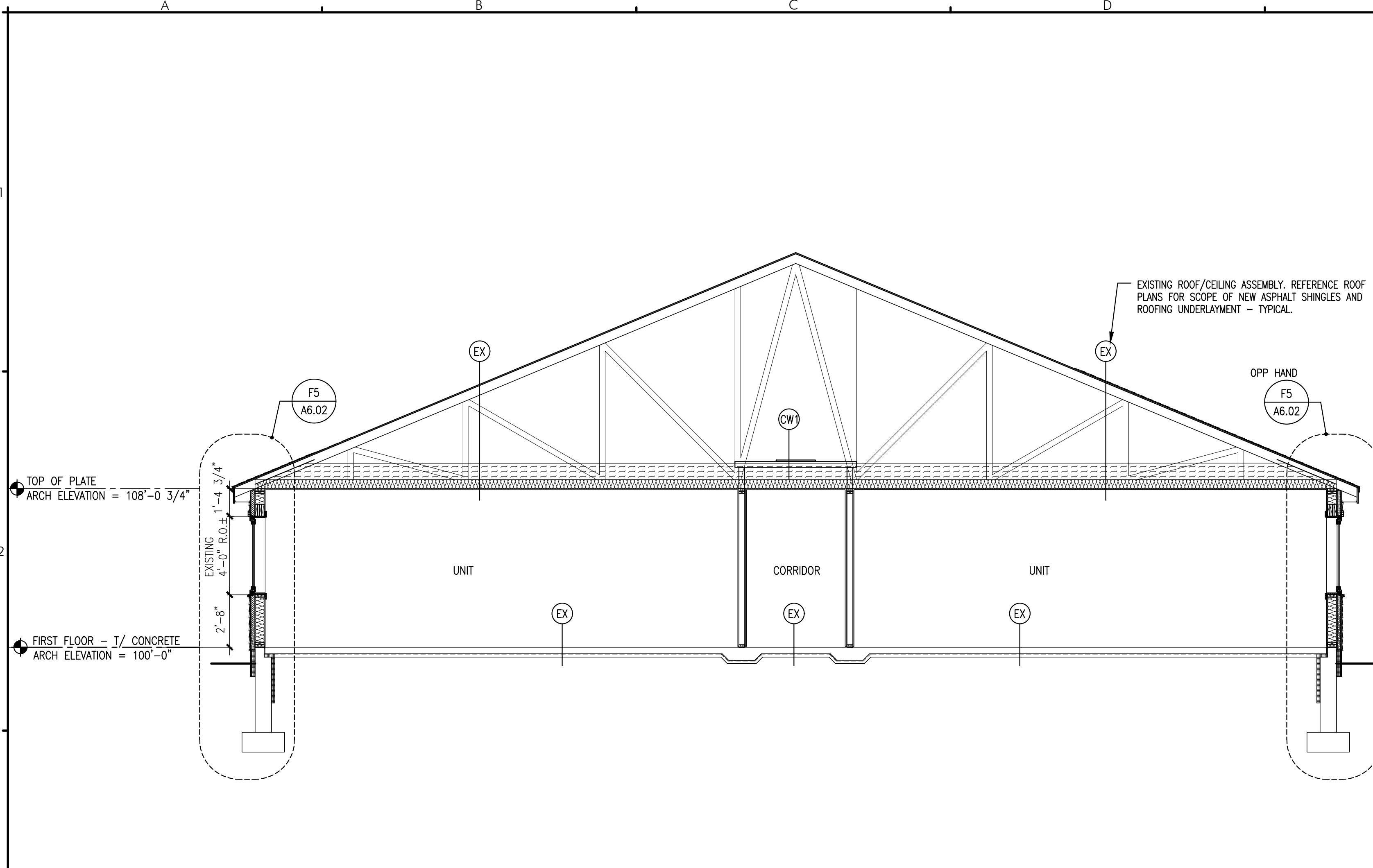
A3 BUILDING SECTION C REFERENCED FROM: SCALE: 1/4" = 1'-0"
