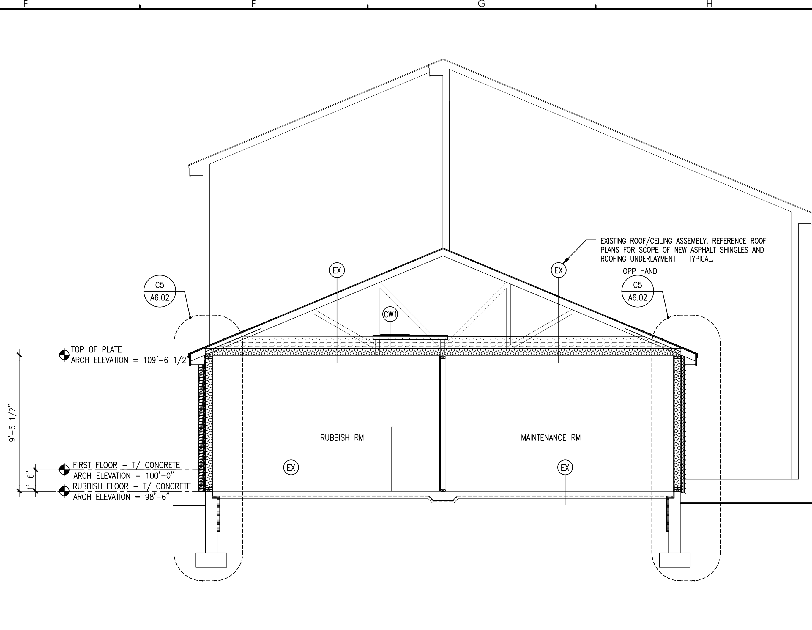
E3 BUILDING SECTION D REFERENCED FROM: SCALE: 1/4" = 1'-0"
