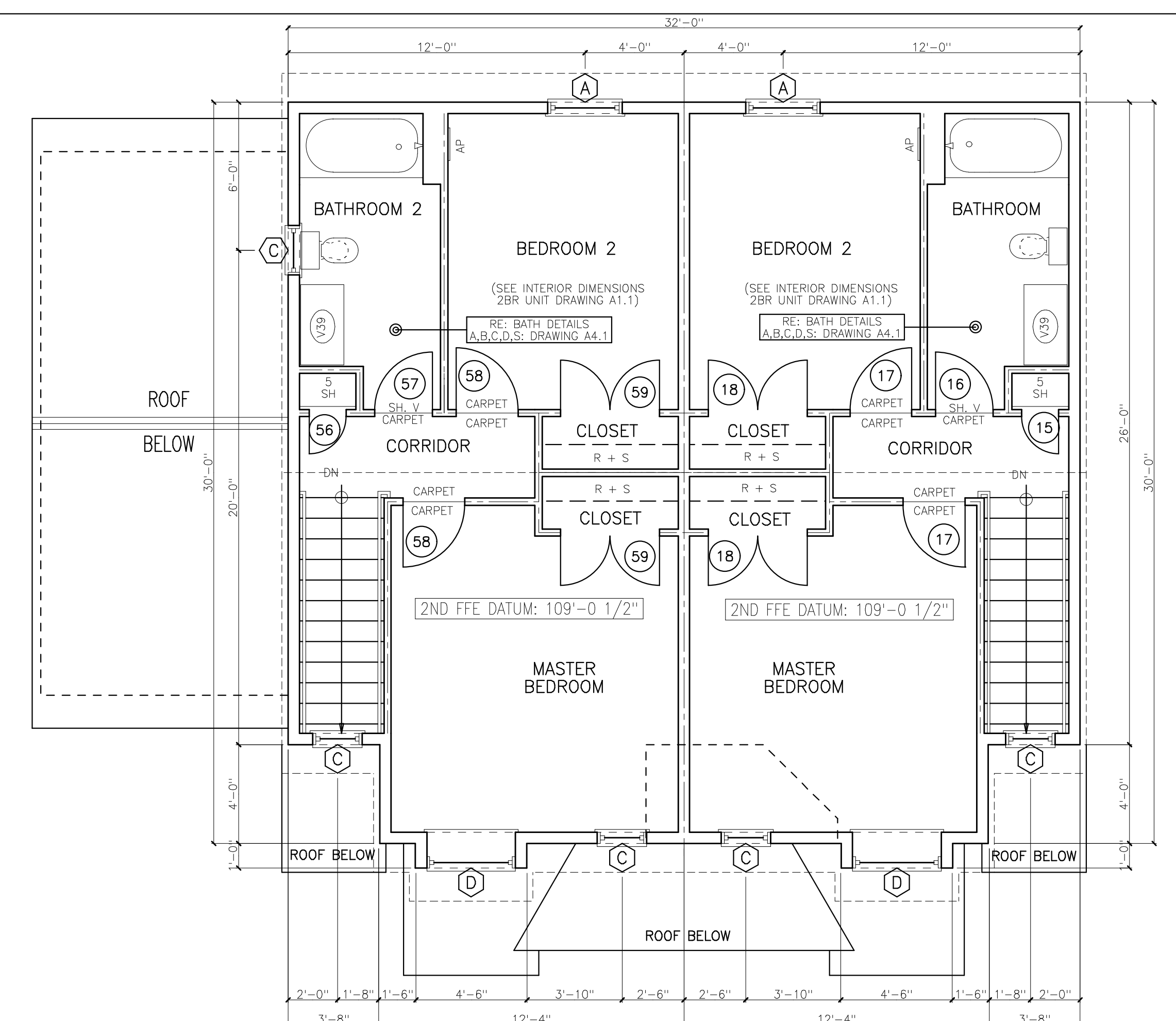
3HCTH/2TH 3BR H.C. TOWNHOUSE/2BR TOWNHOUSE SECOND FLOOR SCALE: 1/4"=1'-0"
