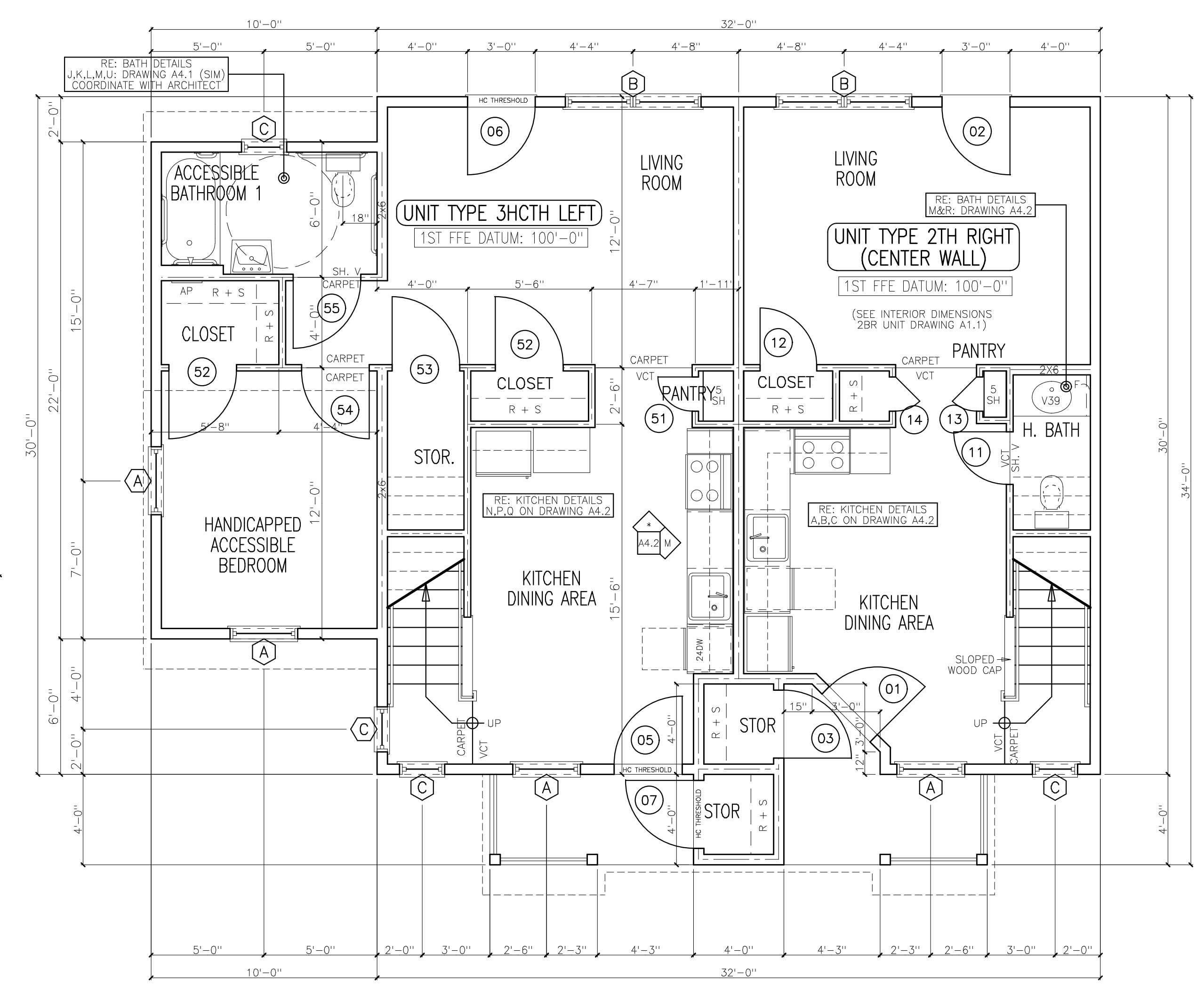
3HCTH/2TH 3BR H.C. TOWNHOUSE/ 2BR TOWNHOUSE FIRST FLOOR SCALE: 1/4"=1'-0"
