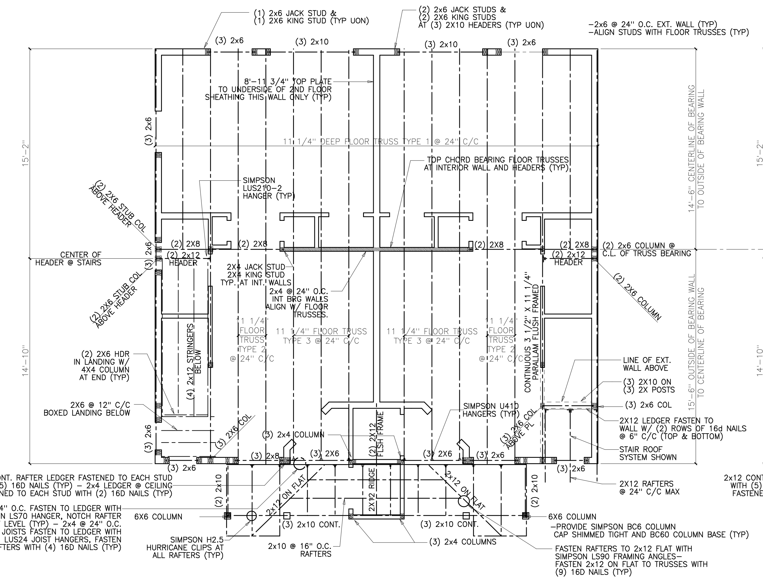
C 2BR TOWNHOUSE 2ND FLOOR FRAMING SCALE: 1/4"=1'-0"
