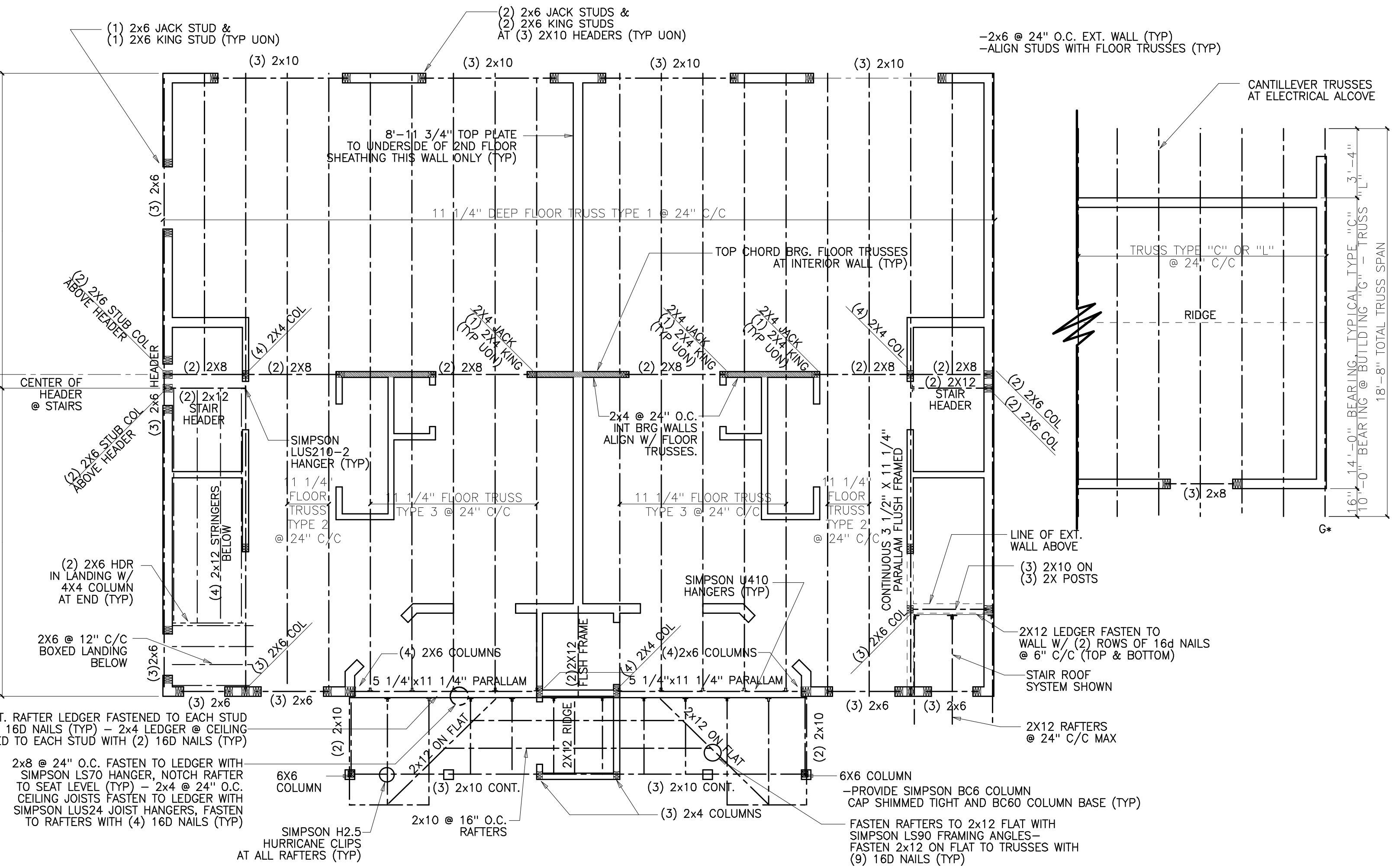
D 3BR TOWNHOUSE 2ND FLOOR FRAMING SCALE: 1/4"=1'-0"
