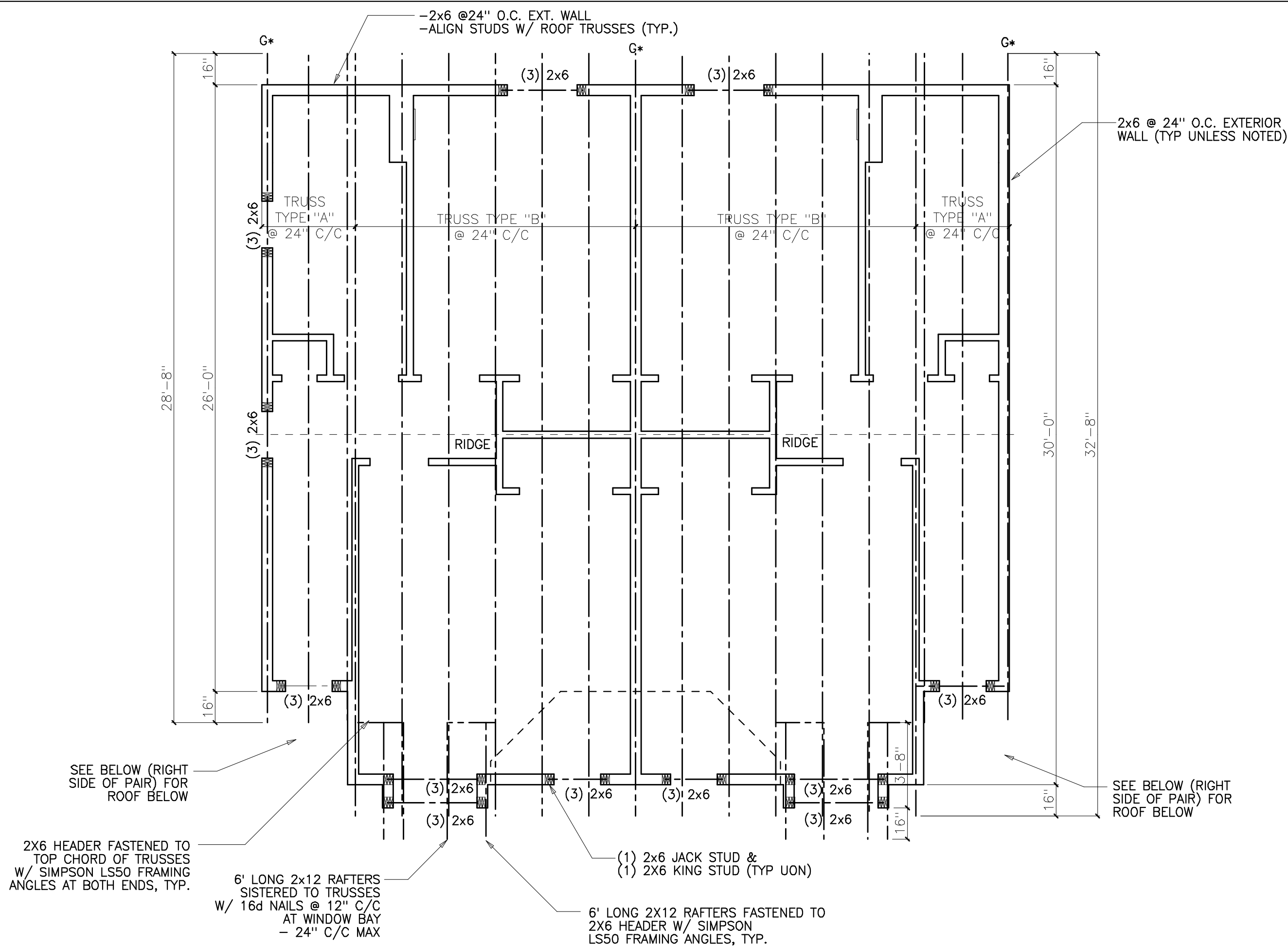
A 2BR TOWNHOUSE ROOF FRAMING SCALE: 1/4"=1'-0"
