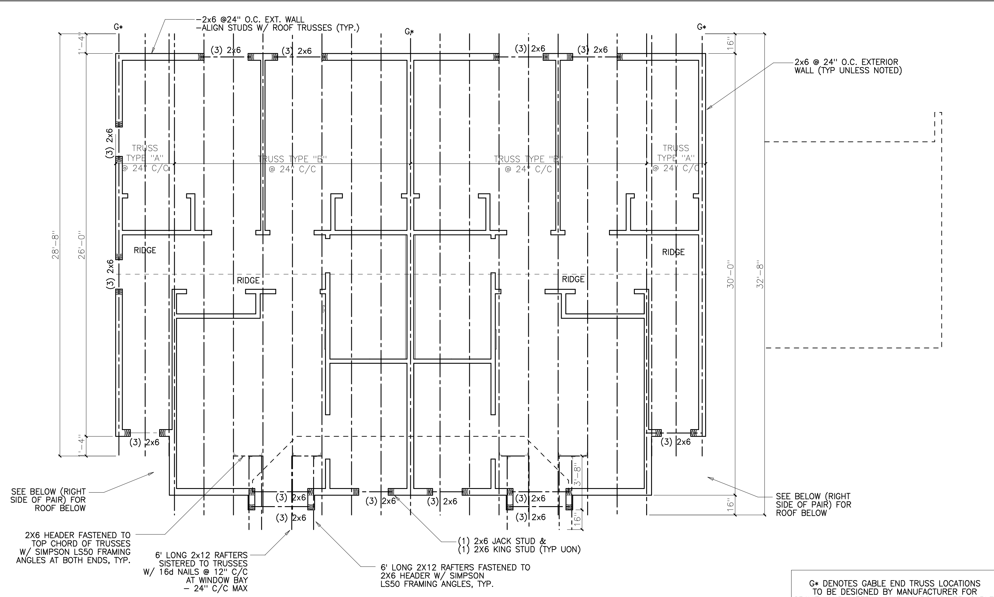
B 3BR TOWNHOUSE ROOF FRAMING SCALE: 1/4"=1'-0"
