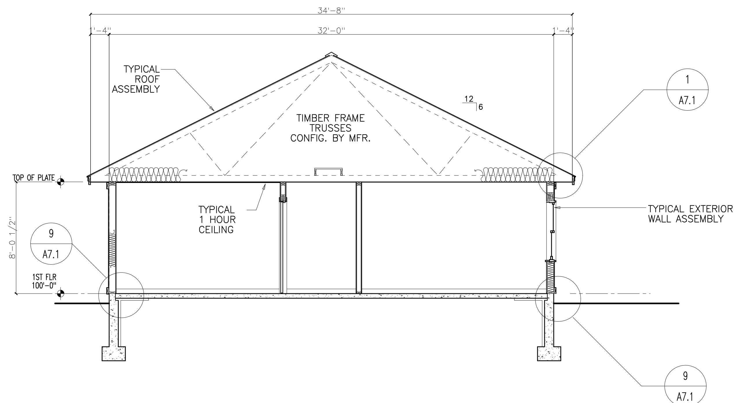
A TYP. HC FLAT BUILDING SECTION SCALE: 1/4"=1'-0"
