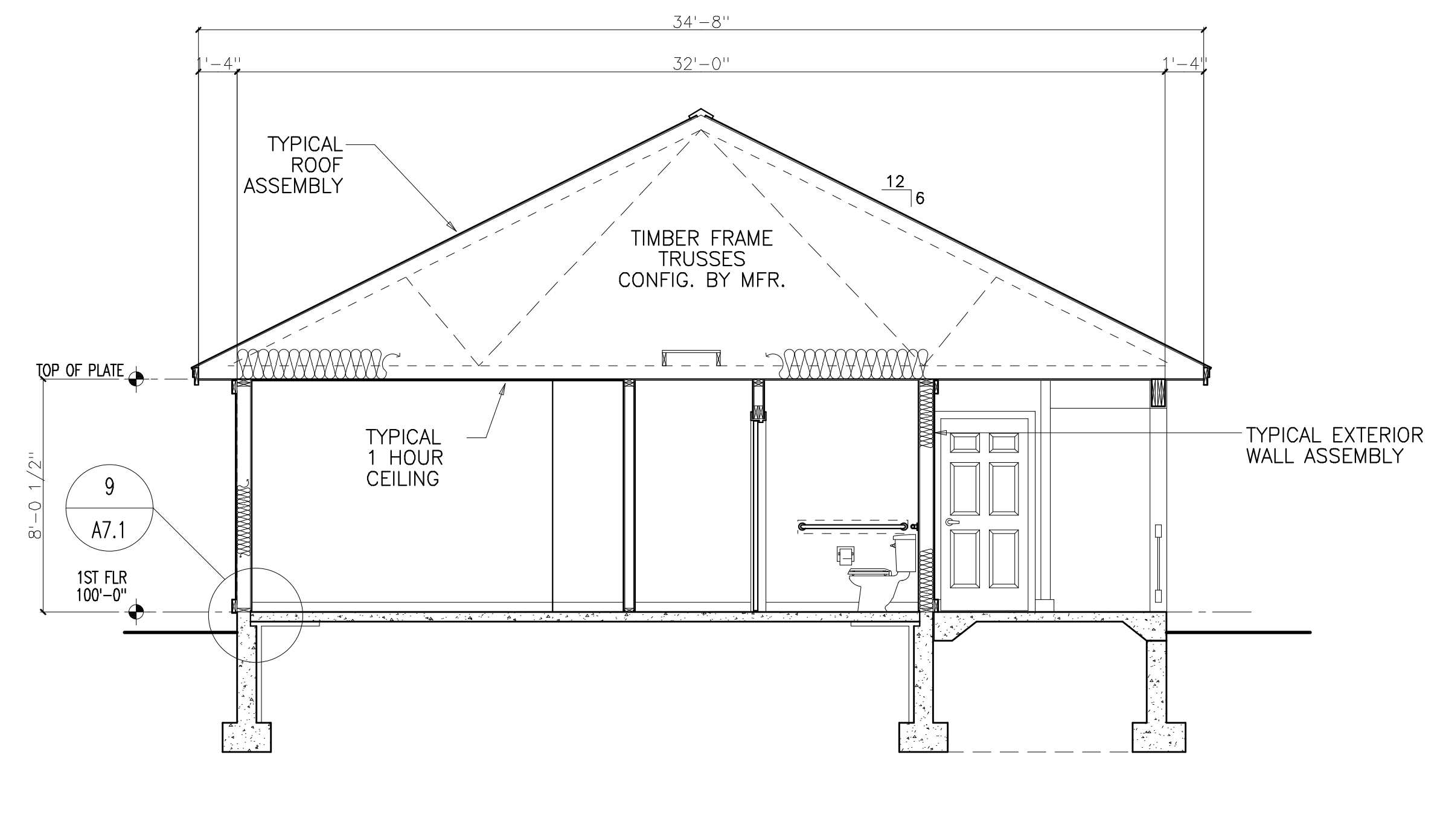
B TYP. HC FLAT BUILDING SECTION SCALE: 1/4"=1'-0"
