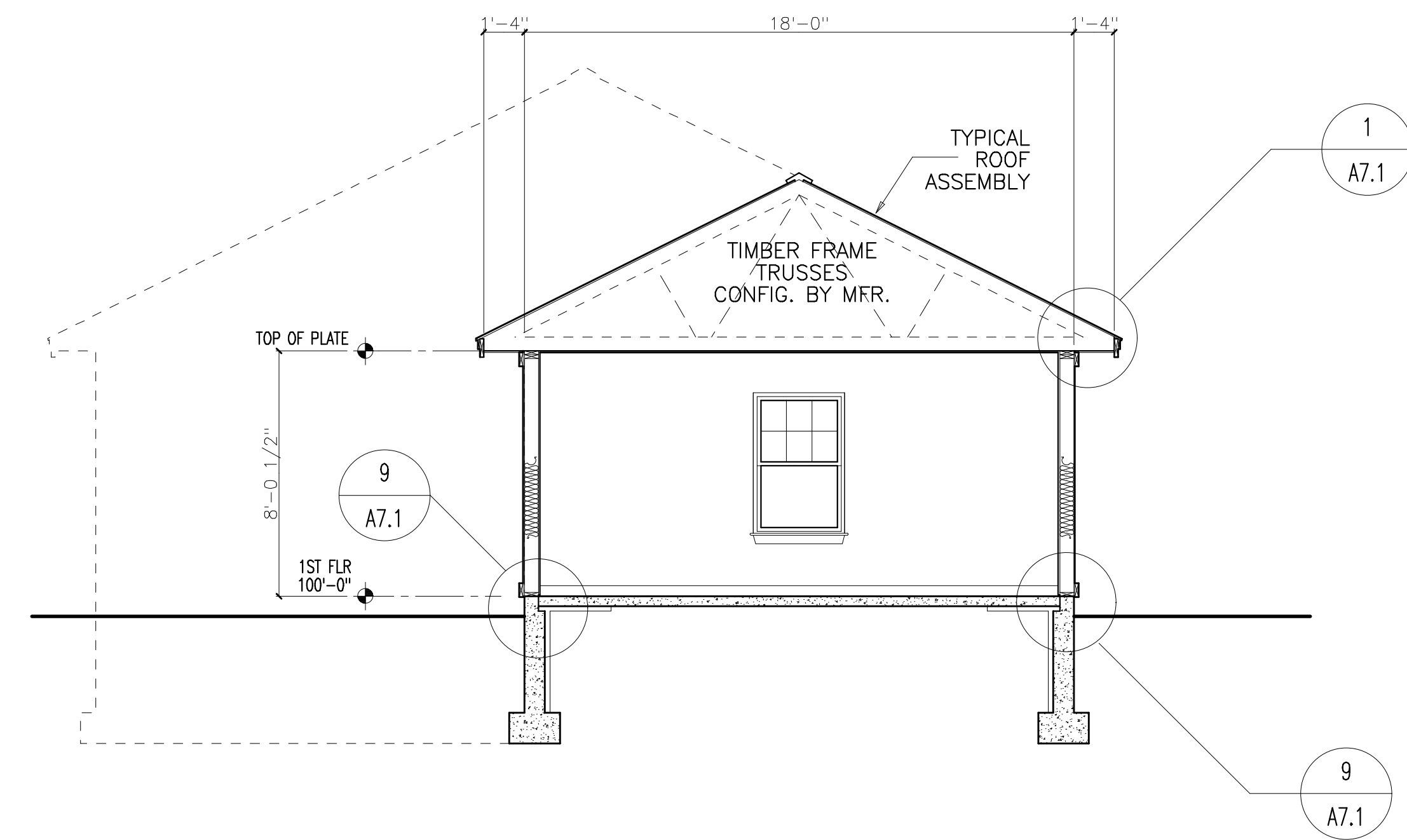
D 3BR HC FLAT BUILDING SECTION SCALE: 1/4"=1'-0"
