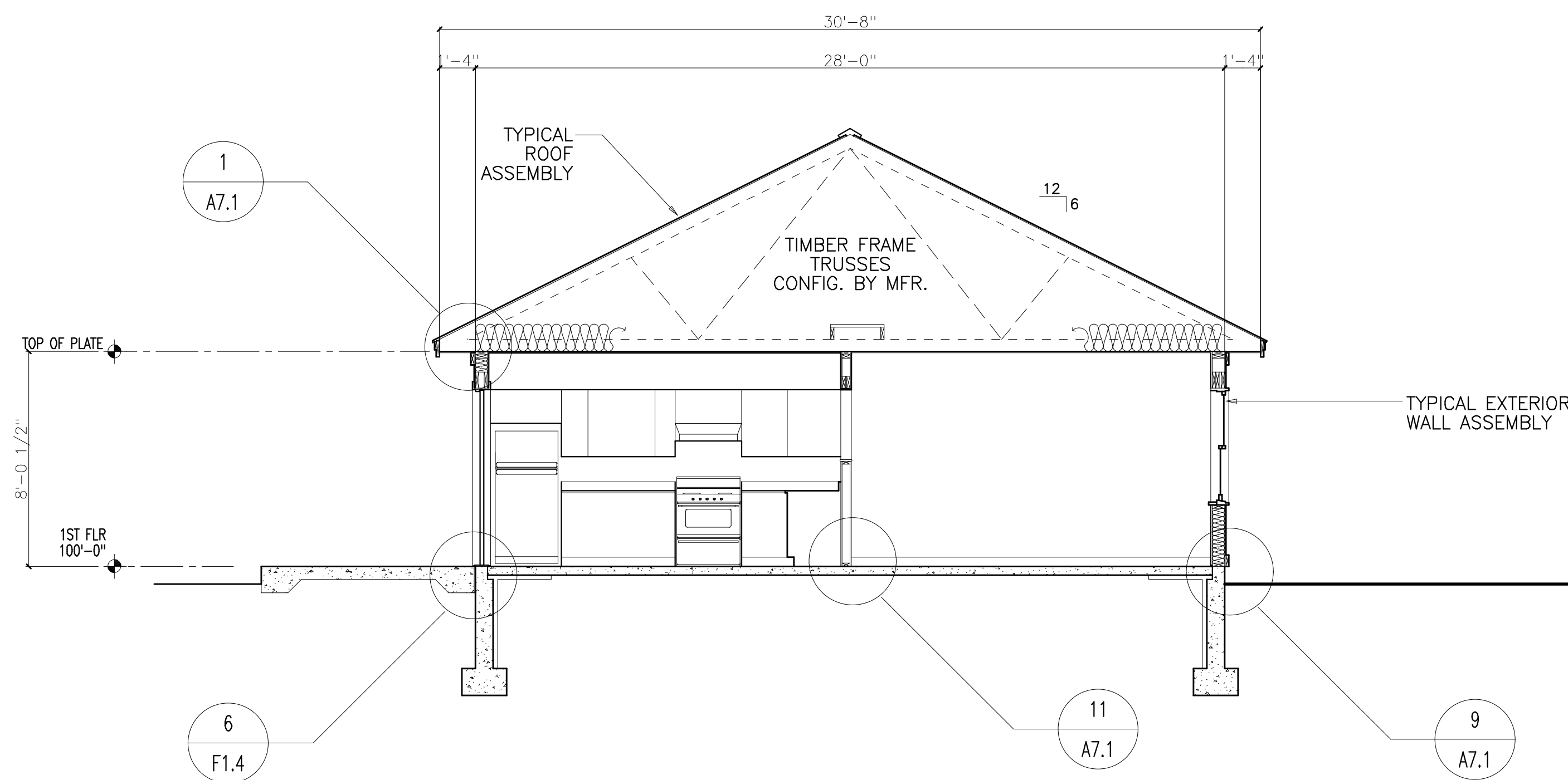
C TYP. HC FLAT BUILDING SECTION SCALE: 1/4"=1'-0"
