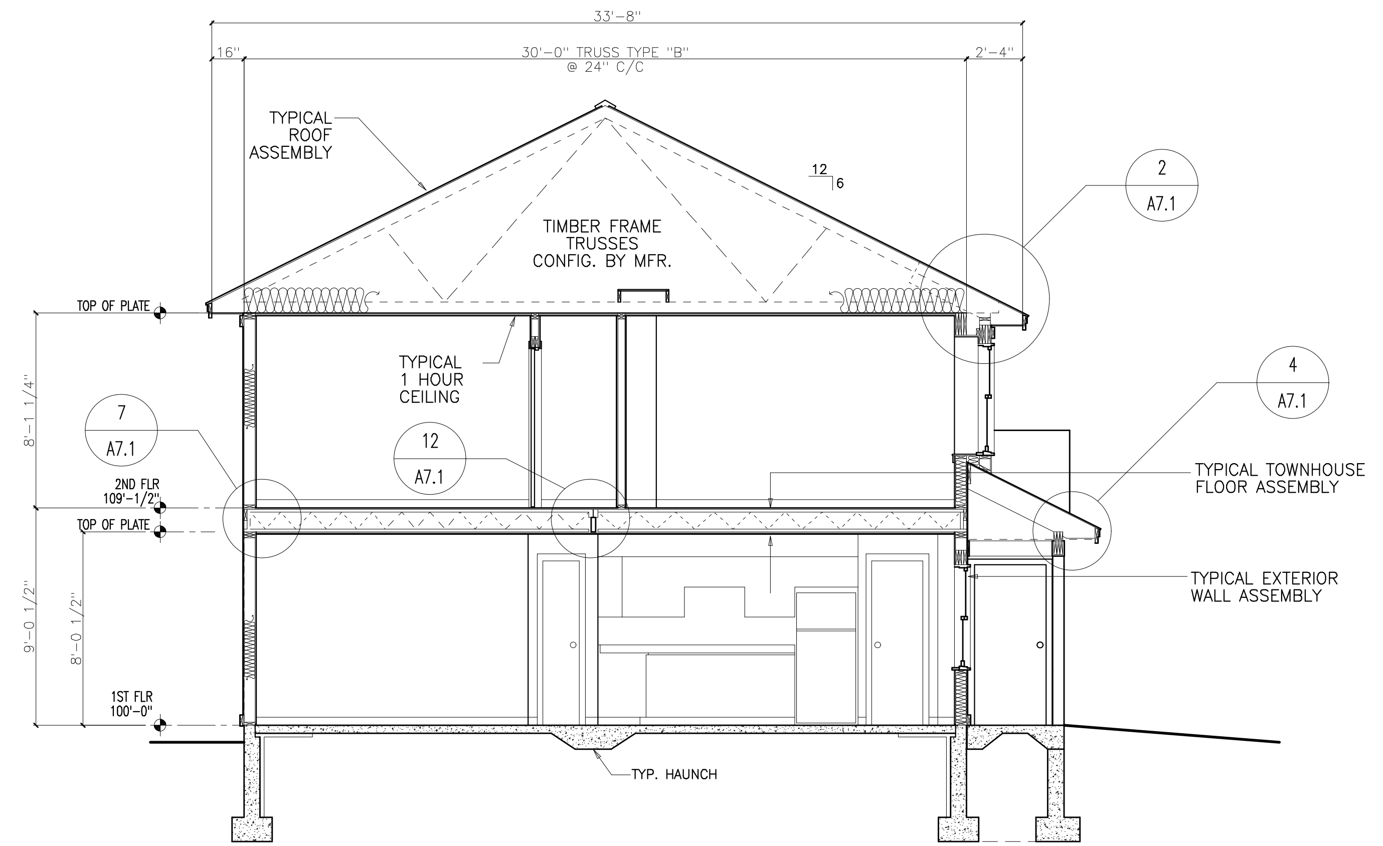
B TYP. 2BR TOWNHOUSE SECTION (3BR. SIM.) SCALE: 1/4"=1'-0"
