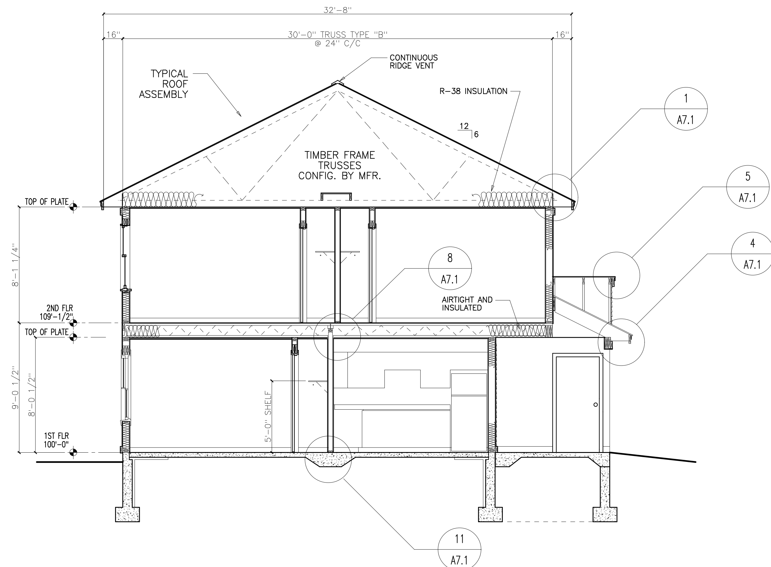
C TYP. 2 BR. TOWNHOUSE SECTION AT PORCH (3 BR. SIM.) SCALE: 1/4"=1'-0"
