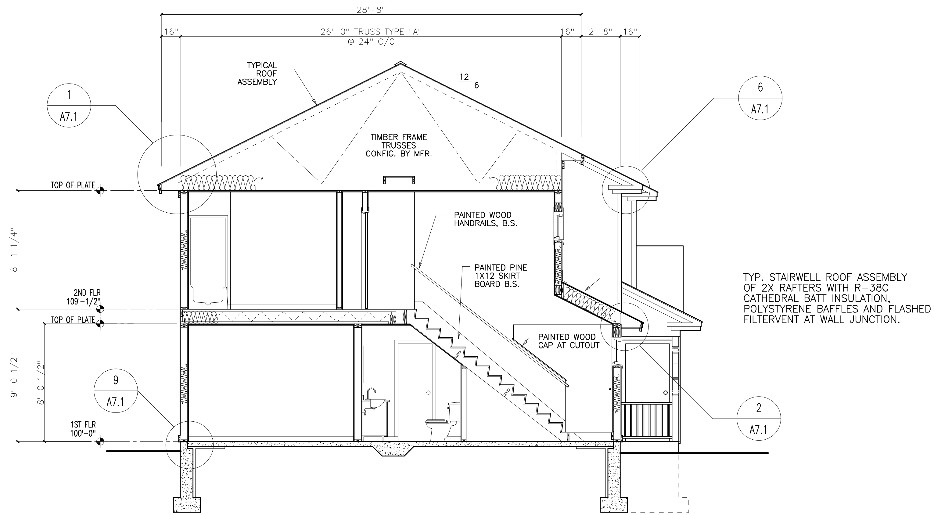
A TYP. 2 BR TOWNHOUSE SECTION AT STAIR (3BR. SIM.) SCALE: 1/4"=1'-0"
