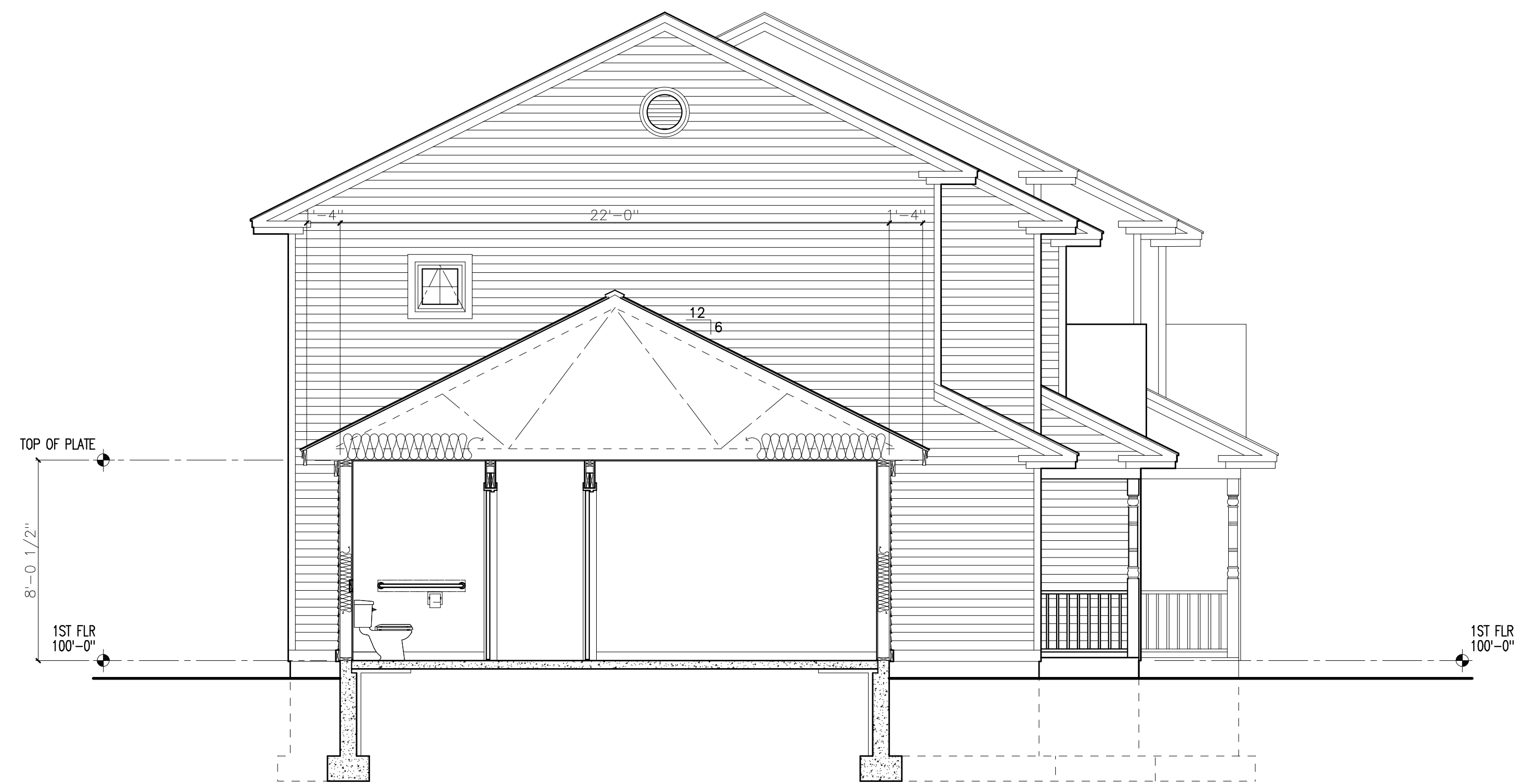
D TYP. BOILER ROOM SECTION SCALE: 1/4"=1'-0"
