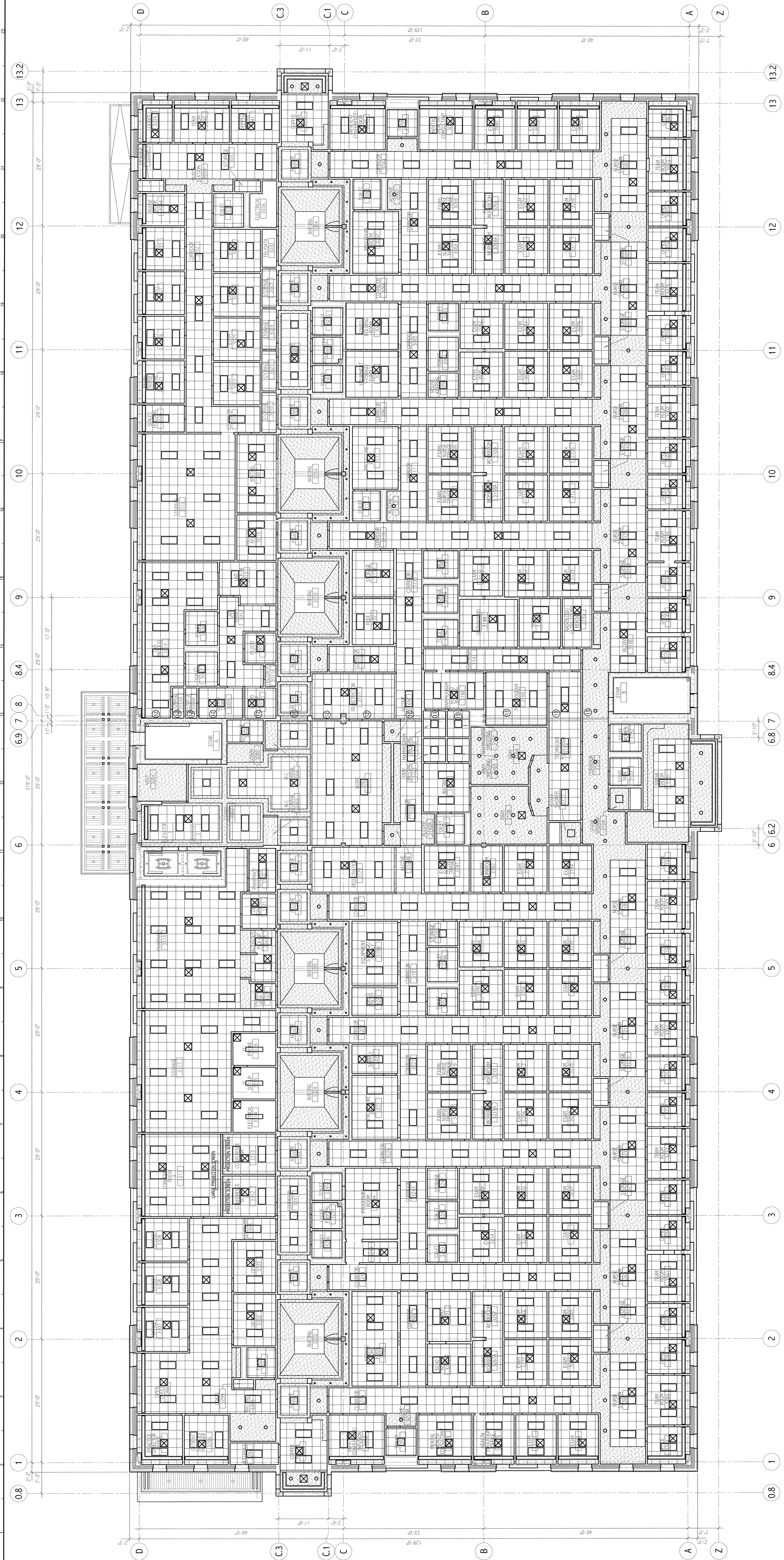
E1 THIRD LEVEL REFLECTED CEILING PLAN 1/8" = 1'-0"
