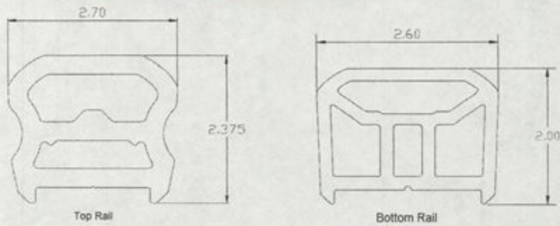
Figure 3 - RadianceRail® Express, Rail Profiles
