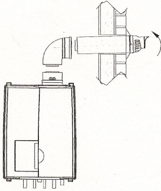
Short termination with wall terminal figure 12A
