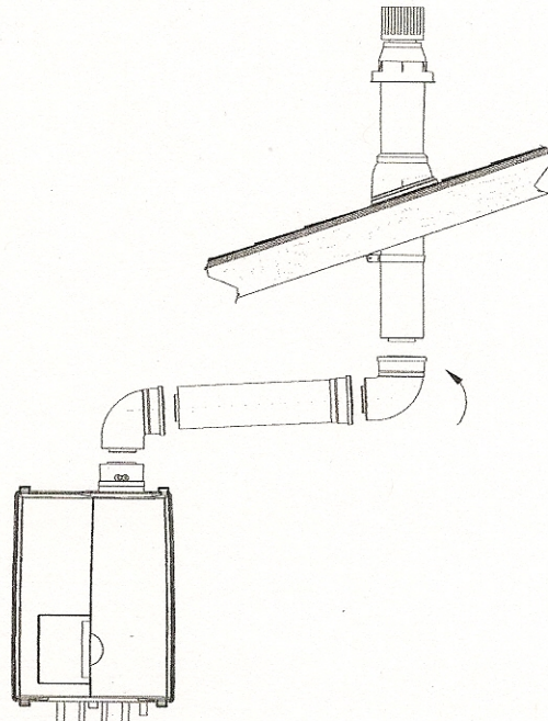
Termination with roof terminal and bends figure 12D
