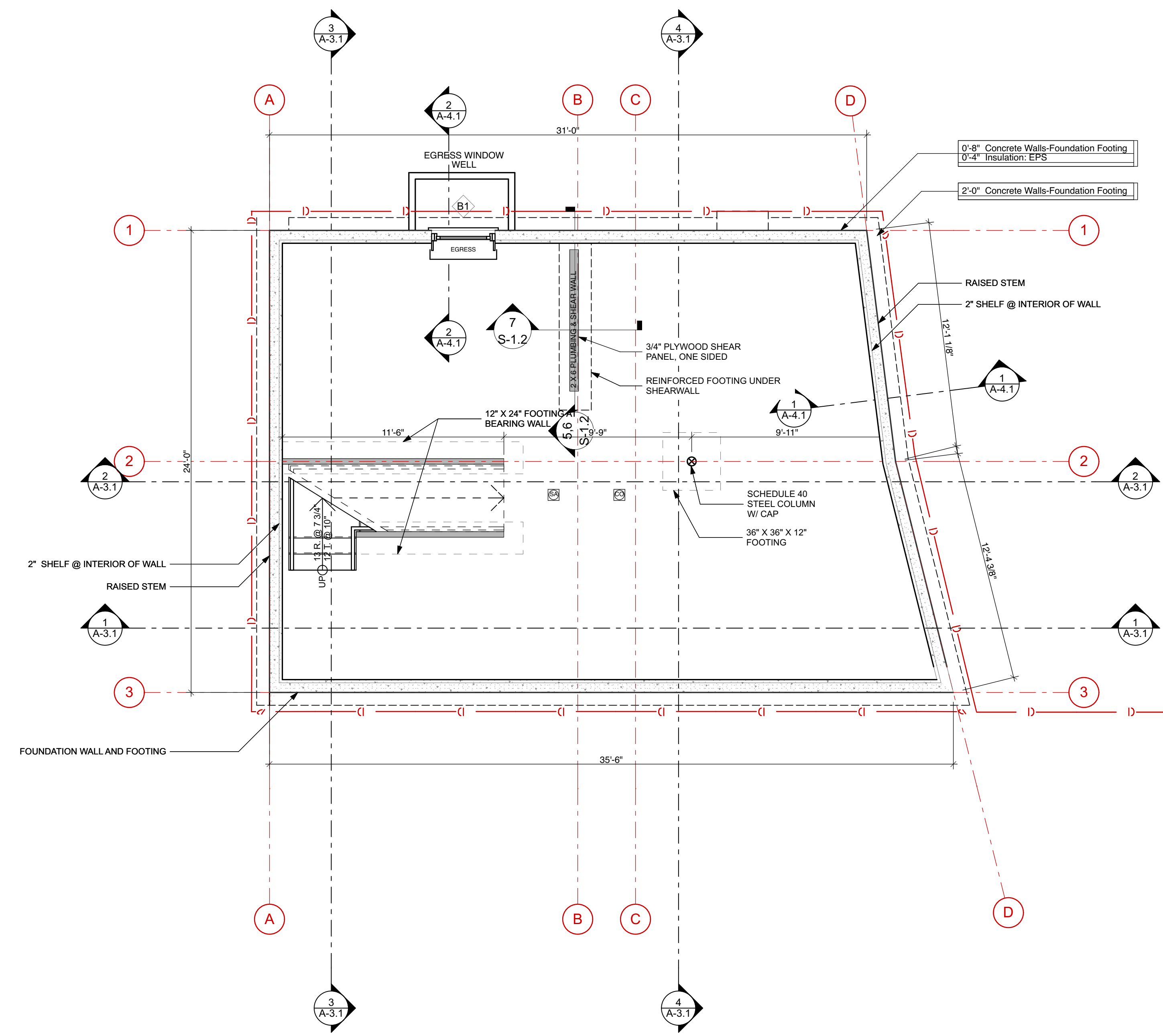
1 BASEMENT SCALE: 1/4" = 1'-0"
