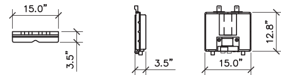
PLAN VIEW SIDE VIEW FRONT VIEW
