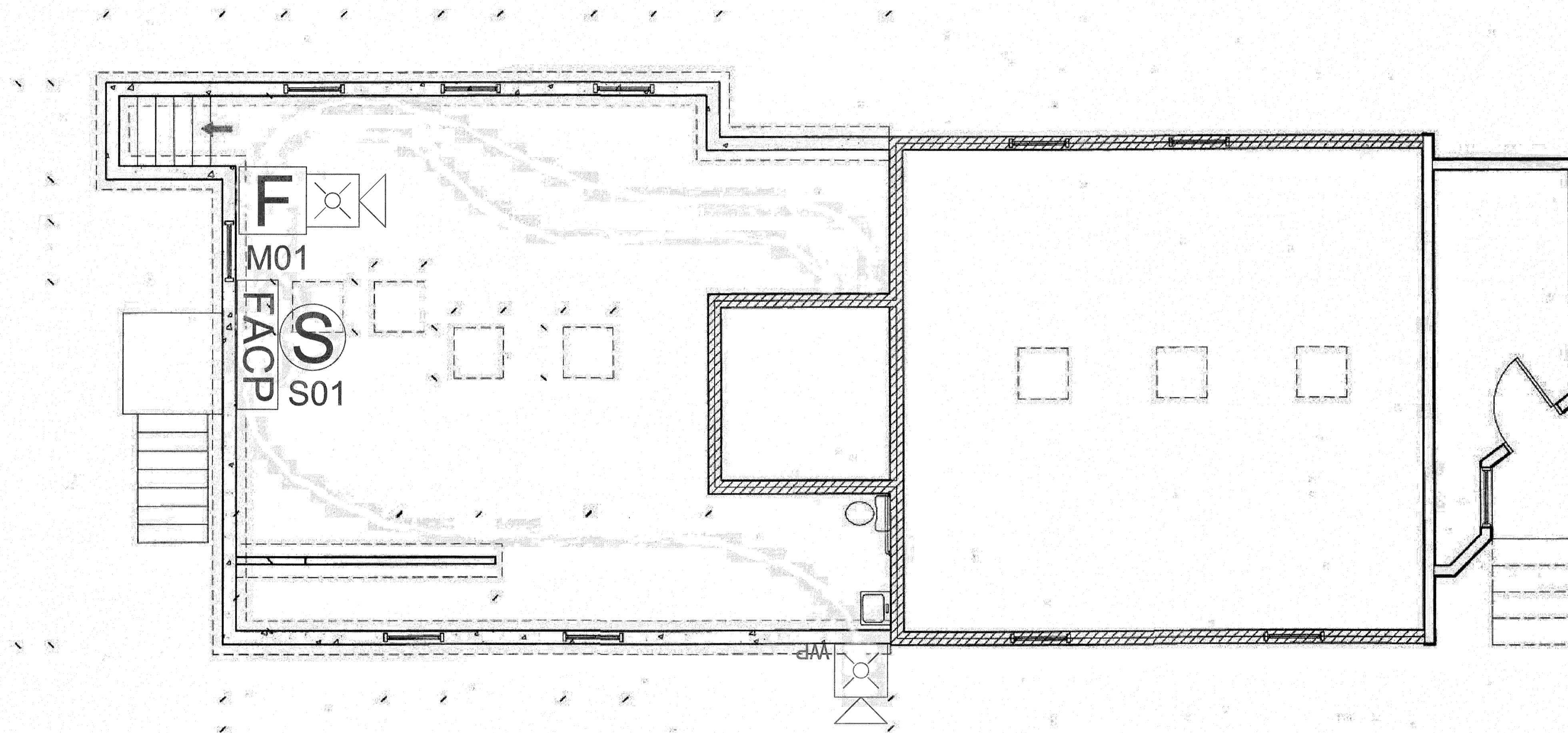
FOUNDATION PLAN
