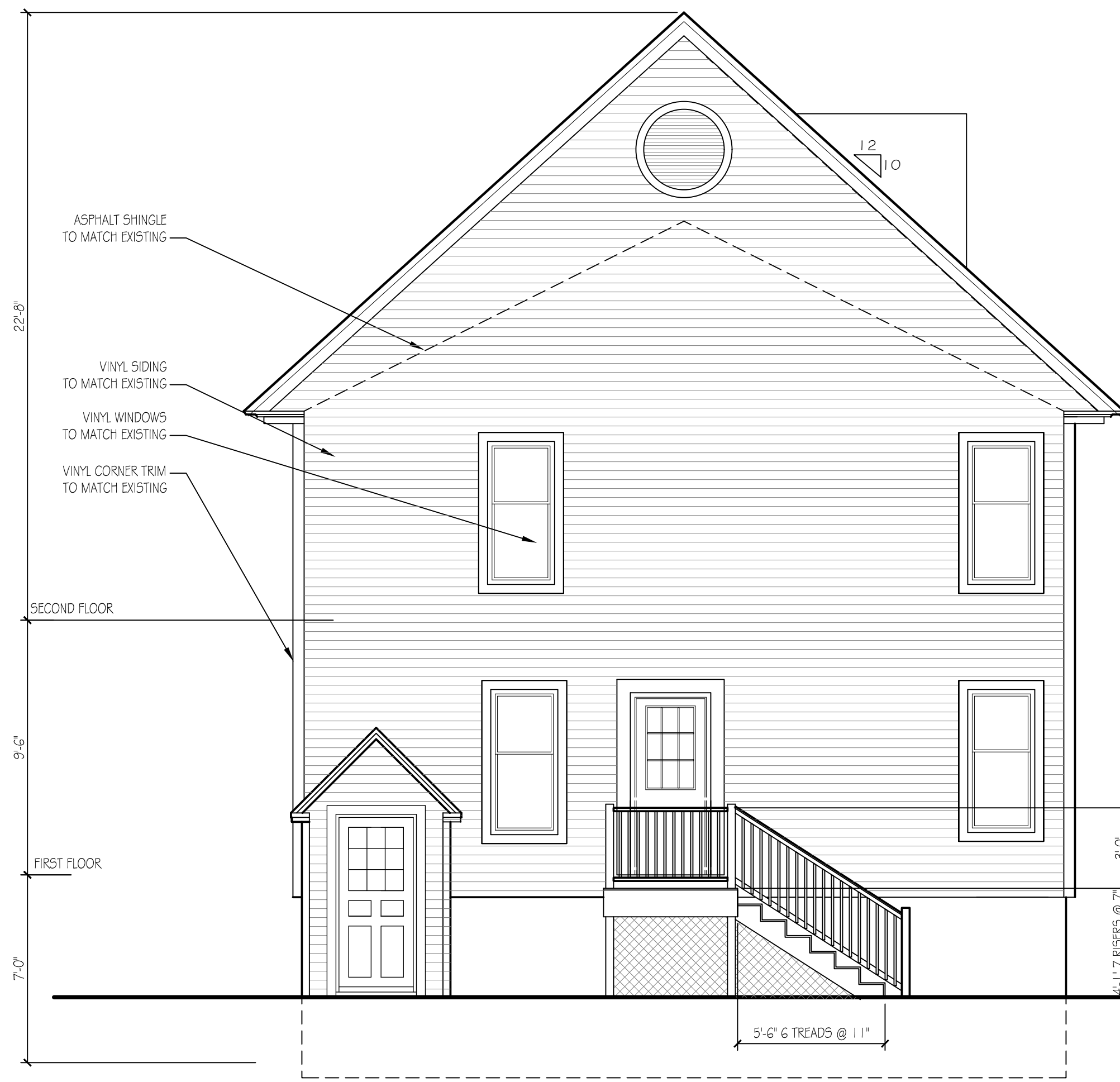
PARKING LOT ELEVATION SCALE: 1/4"=1'-0"
