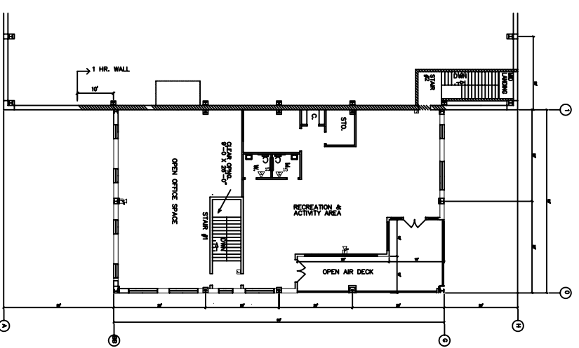
SECOND FLOOR OFFICE / SERVICE BUILDING
