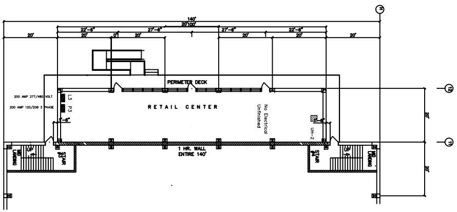
SECOND FLOOR RETAIL BUILDING
