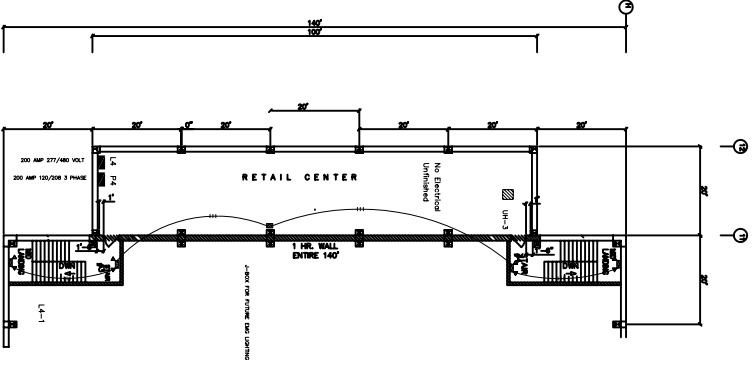
THIRD FLOOR RETAIL BUILDING
