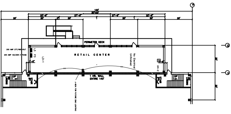
SECOND FLOOR RETAIL BUILDING
