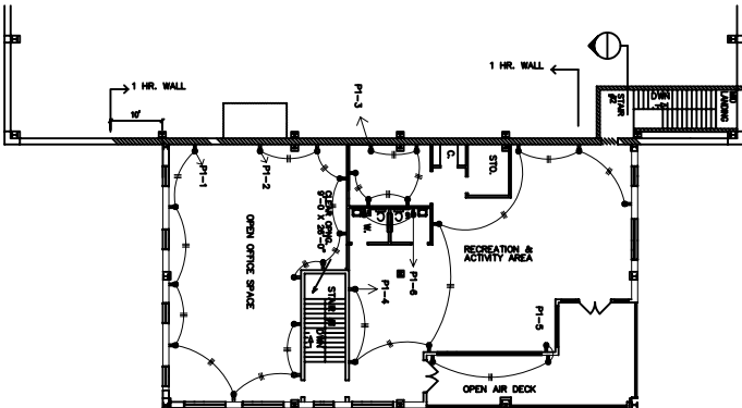
SECOND FLOOR OFFICE / SERVICE BUILDING
