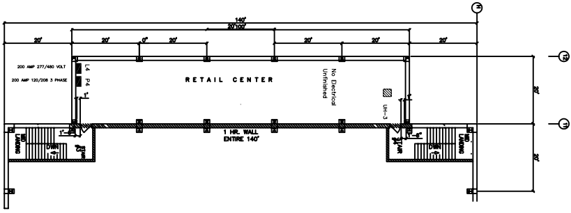
THIRD FLOOR RETAIL BUILDING
