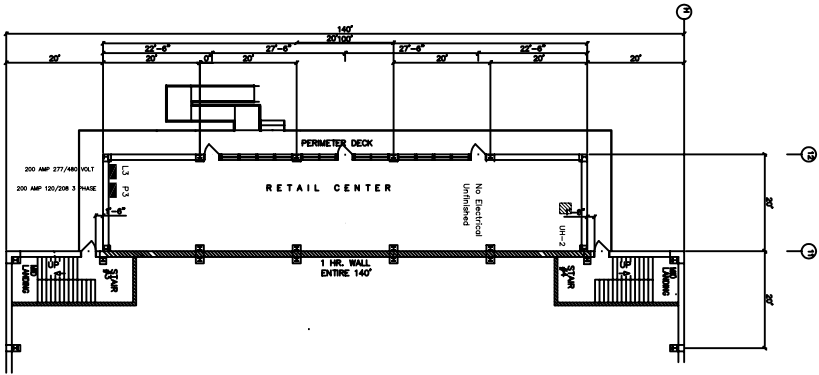
SECOND FLOOR RETAIL BUILDING
