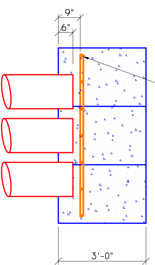
P.C. SECTION 3 1/2" = 1'-0"
