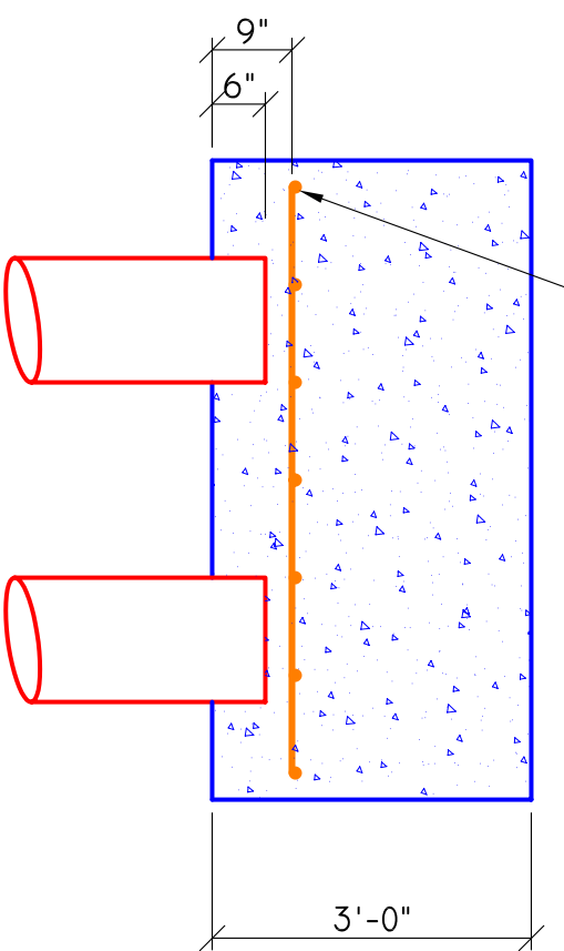
P.C. SECTION 2 1/2" = 1'-0"
