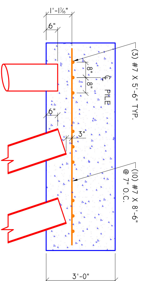
P.C. SECTION 7 1/2" = 1'-0"
