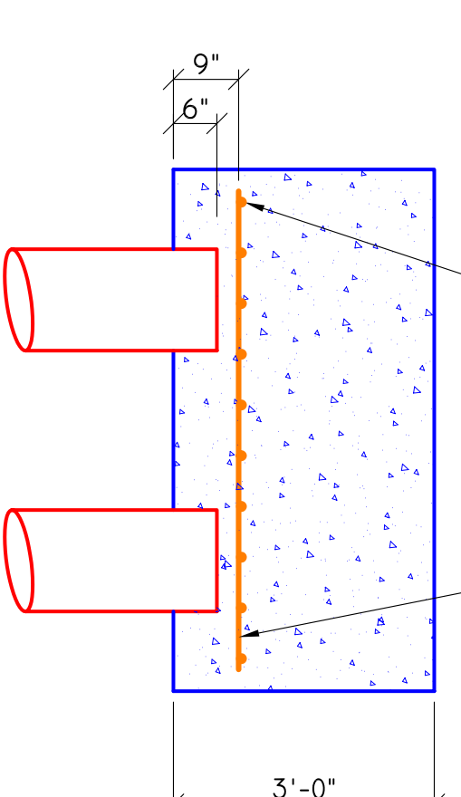
P.C. SECTION 5 1/2" = 1'-0"
