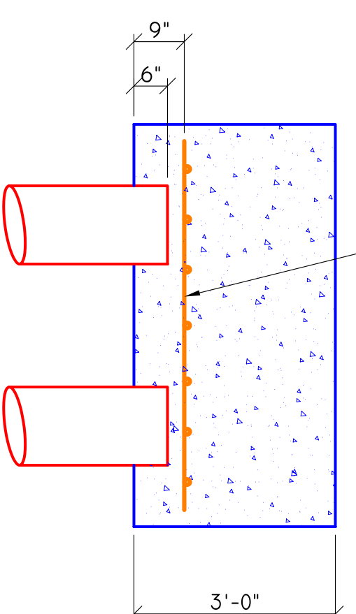
P.C. SECTION 4 1/2" = 1'-0"
