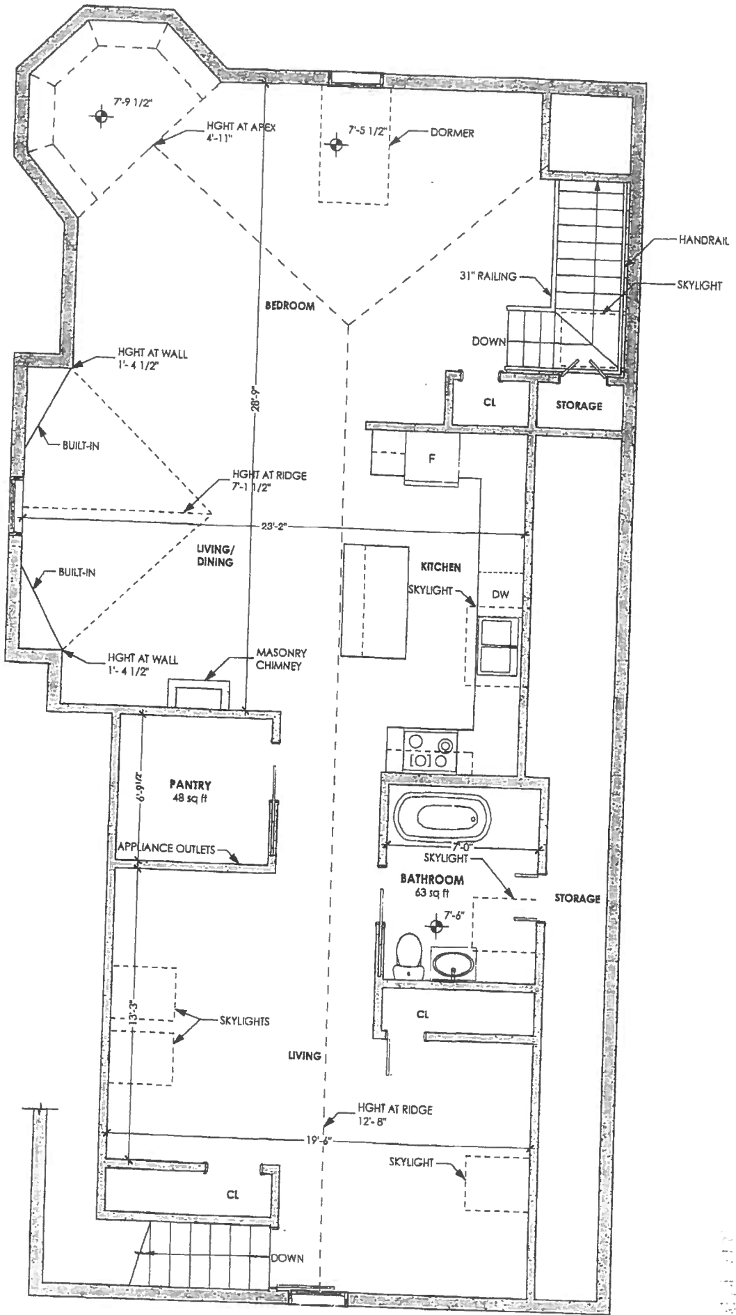
613 WASHINGTON STREET- UNIT 3 EXISTING PLAN SCALE: 1/4" = 1'-0"
