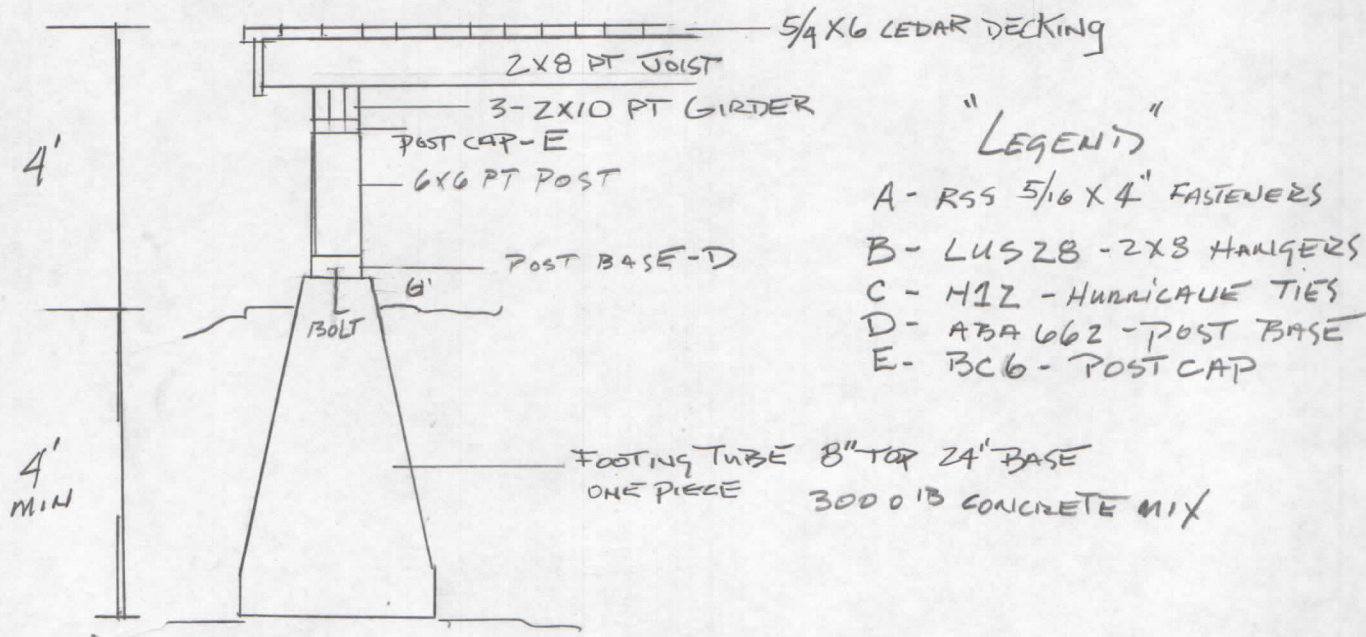
S-1 FOUNDATION PLAN FRAMING SECTION & DETAIL
