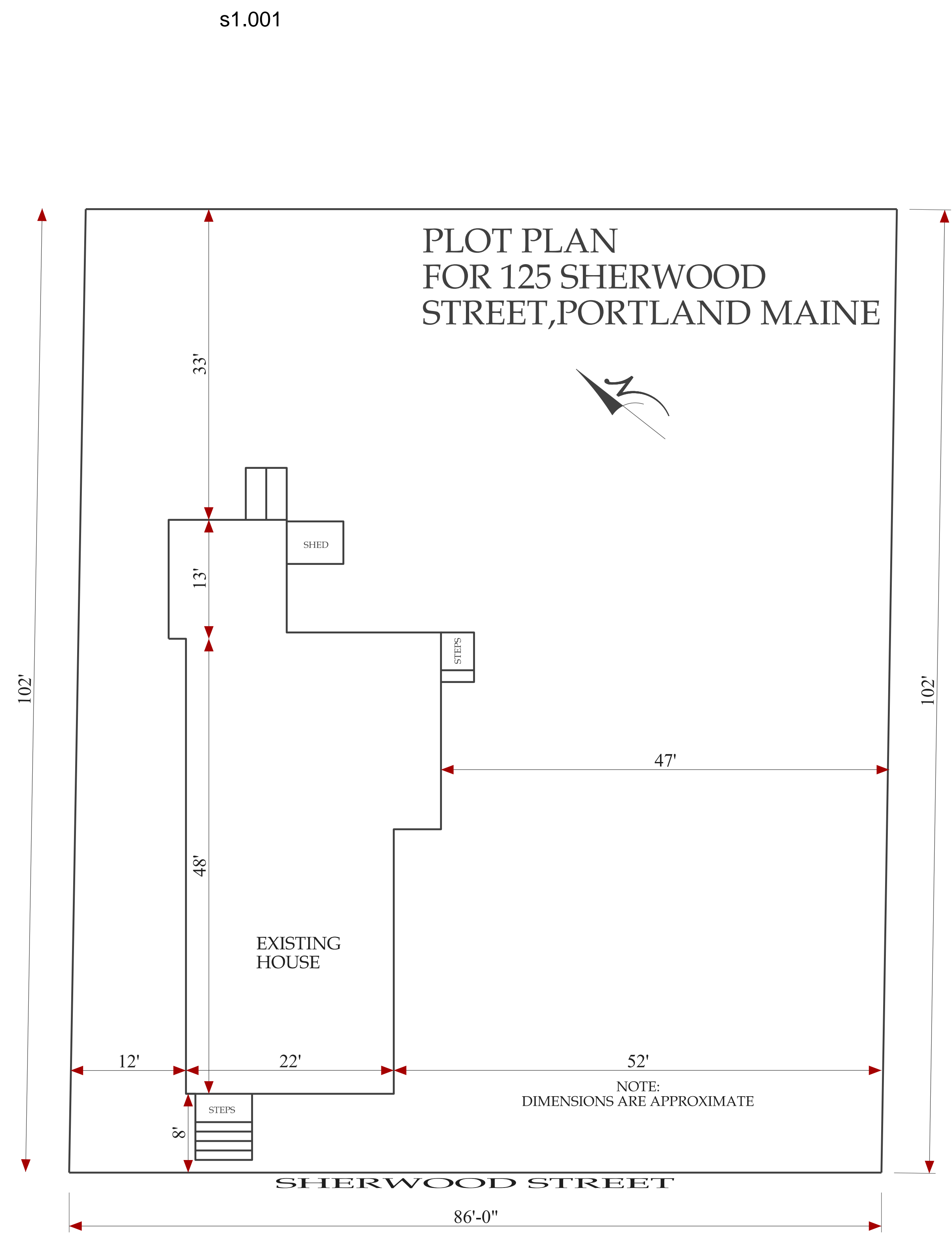
PLOT PLAN SCALE 1/8"=1'-0"
