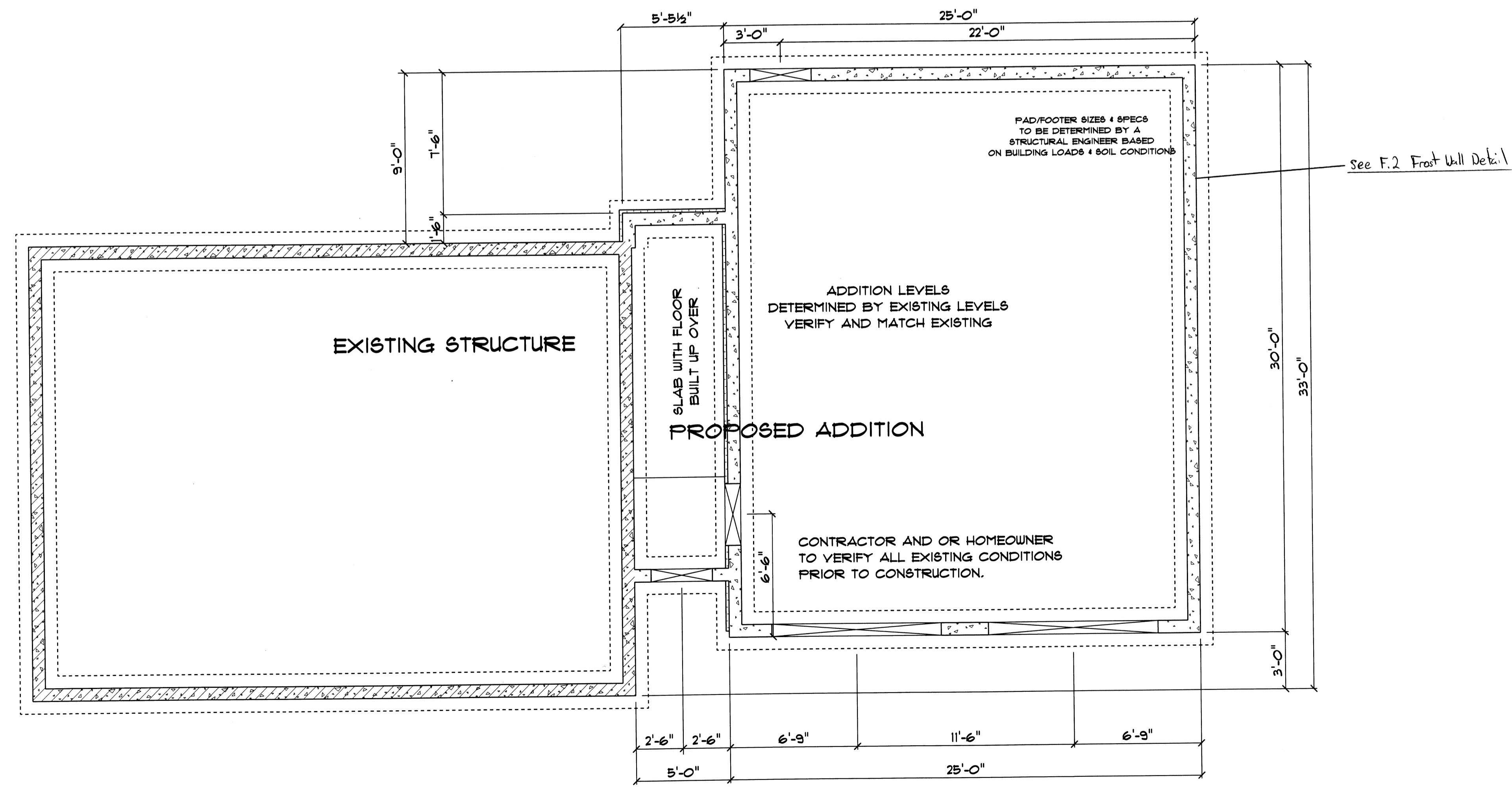
FOUNDATION SCALE: 1/4" = 1'-0"
